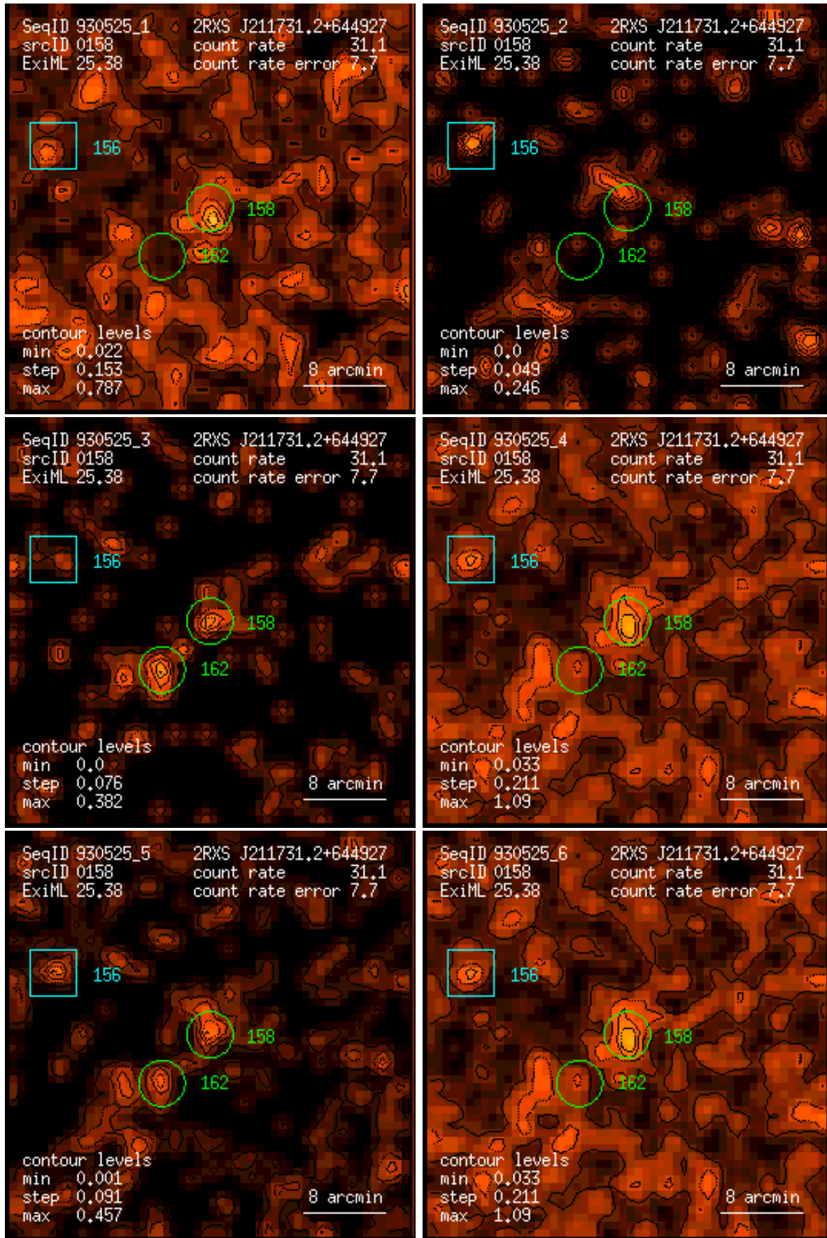
Figure 158: RASS 930525: detection 0158: band rate images, Gaussian filter: (1) PSPC channels 11 – 41, (2) 52 – 90, (3) 91 – 201, (4) 11 – 235, (5) 52 – 201, (6) 11 – 201. Broad band rates in counts/ks. Band rate contour levels in counts/ks/arcmin 2 .
