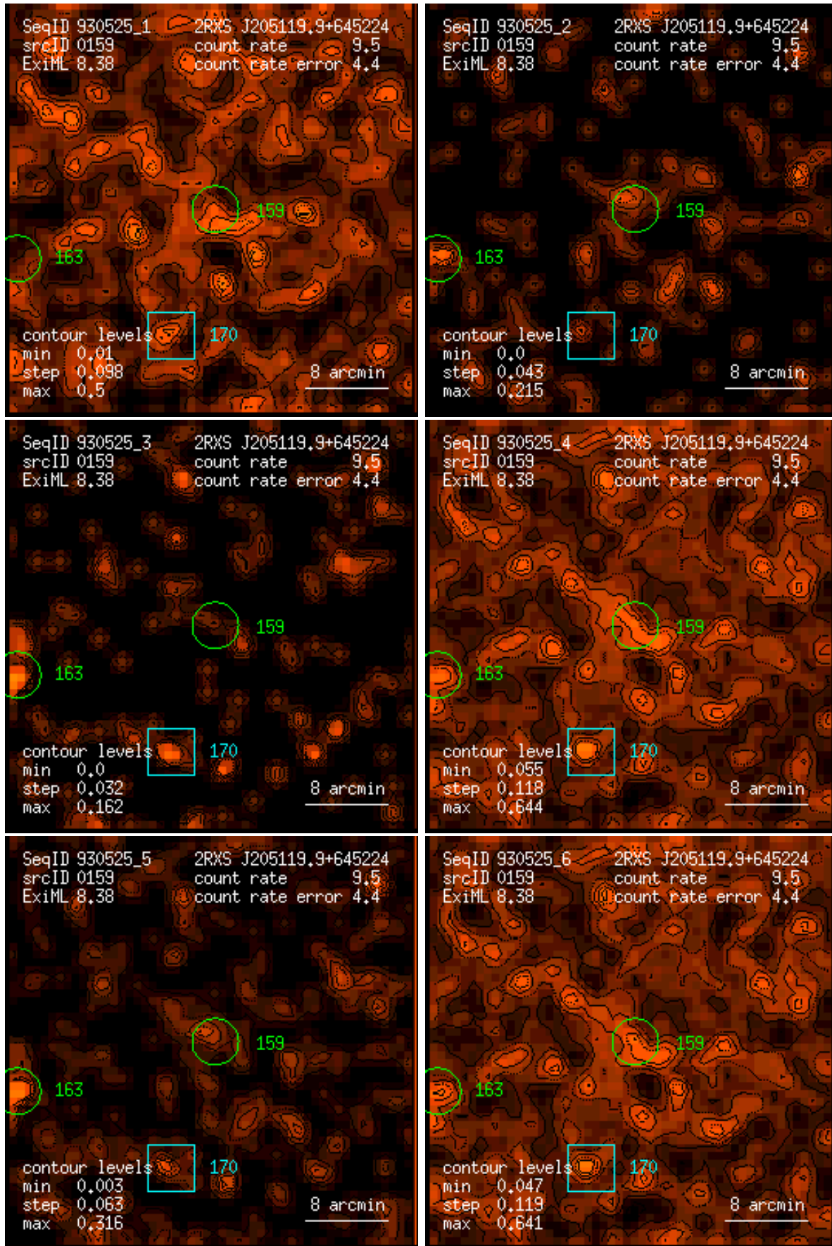
Figure 159: RASS 930525: detection 0159: band rate images, Gaussian filter: (1) PSPC channels 11 – 41, (2) 52 – 90, (3) 91 – 201, (4) 11 – 235, (5) 52 – 201, (6) 11 – 201. Broad band rates in counts/ks. Band rate contour levels in counts/ks/arcmin 2 .
