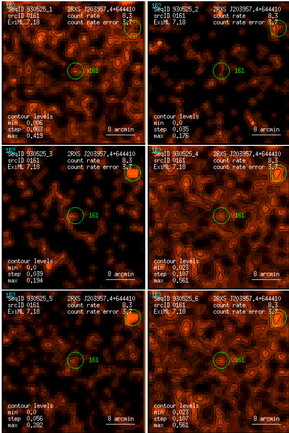
Figure 161: RASS 930525: detection 0161: band rate images, Gaussian filter: (1) PSPC channels 11 – 41, (2) 52 – 90, (3) 91 – 201, (4) 11 – 235, (5) 52 – 201, (6) 11 – 201. Broad band rates in counts/ks. Band rate contour levels in counts/ks/arcmin 2 .
