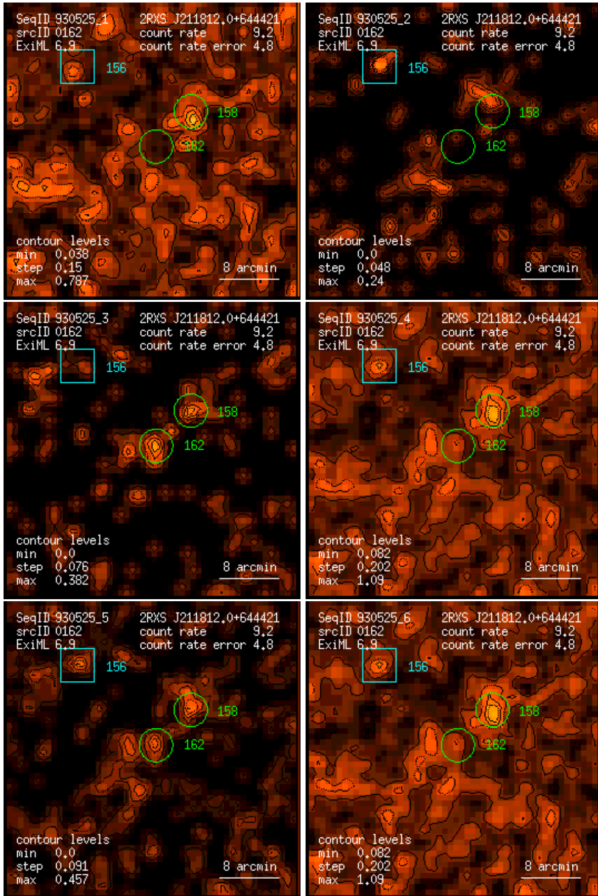
Figure 162: RASS 930525: detection 0162: band rate images, Gaussian filter: (1) PSPC channels 11 – 41, (2) 52 – 90, (3) 91 – 201, (4) 11 – 235, (5) 52 – 201, (6) 11 – 201. Broad band rates in counts/ks. Band rate contour levels in counts/ks/arcmin 2 .
