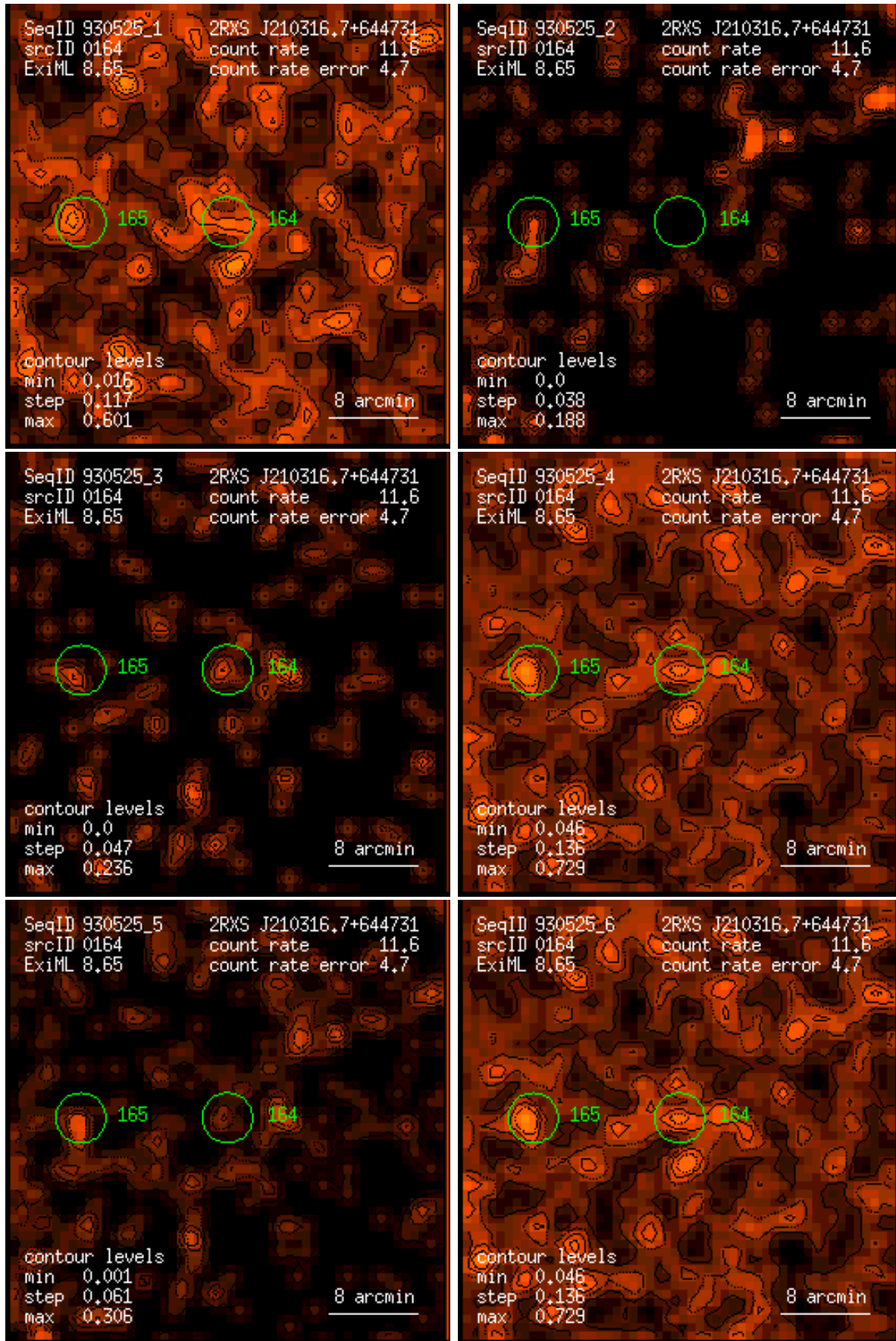
Figure 164: RASS 930525: detection 0164: band rate images, Gaussian filter: (1) PSPC channels 11 – 41, (2) 52 – 90, (3) 91 – 201, (4) 11 – 235, (5) 52 – 201, (6) 11 – 201. Broad band rates in counts/ks. Band rate contour levels in counts/ks/arcmin 2 .
