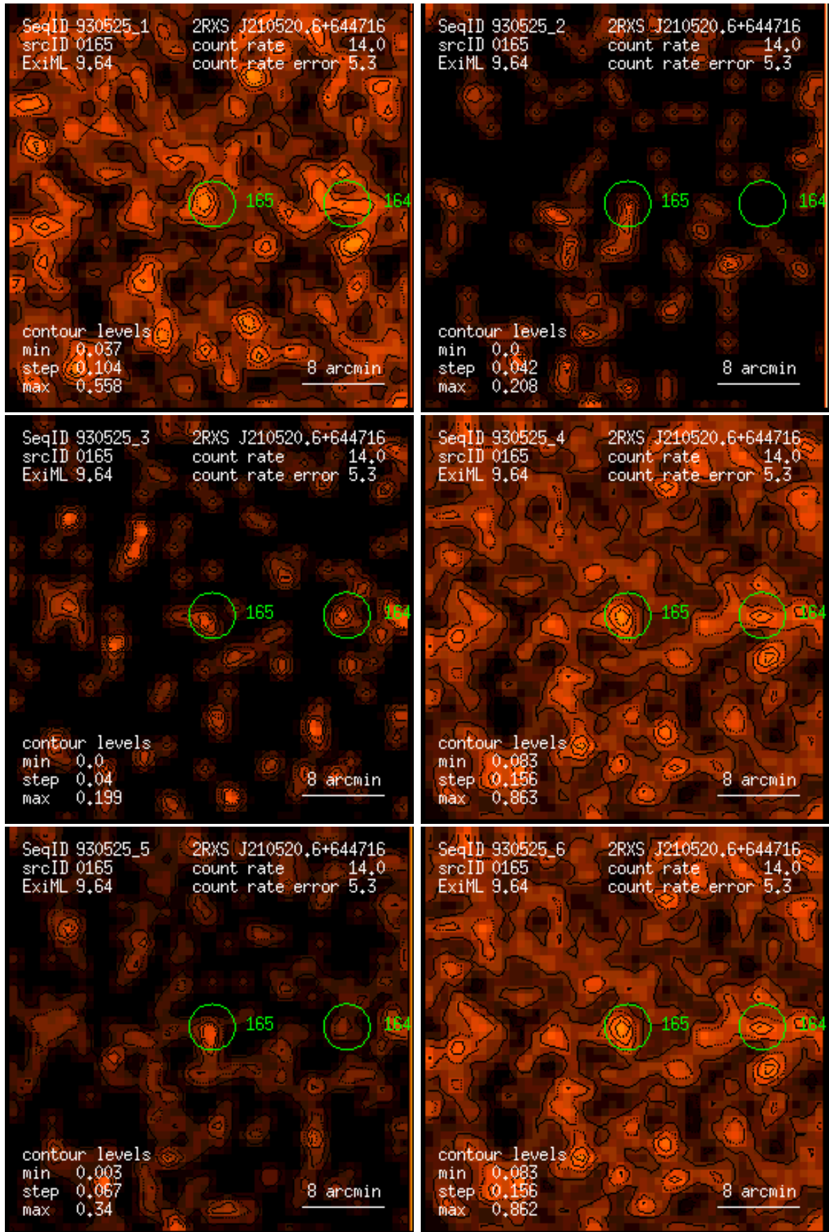
Figure 165: RASS 930525: detection 0165: band rate images, Gaussian filter: (1) PSPC channels 11 – 41, (2) 52 – 90, (3) 91 – 201, (4) 11 – 235, (5) 52 – 201, (6) 11 – 201. Broad band rates in counts/ks. Band rate contour levels in counts/ks/arcmin 2 .
