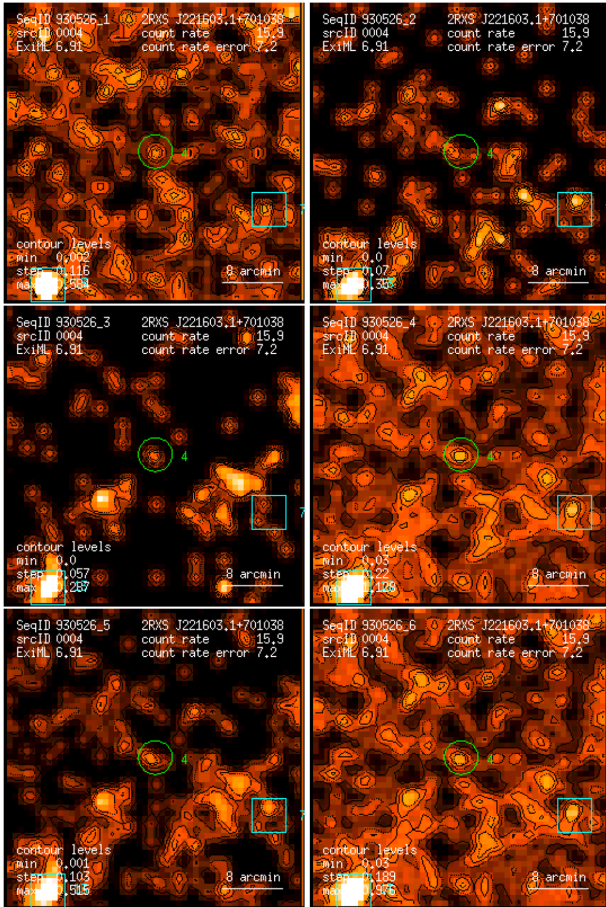
Figure 4: RASS 930526: detection 0004: band rate images, Gaussian filter: (1) PSPC channels 11 – 41, (2) 52 – 90, (3) 91 – 201, (4) 11 – 235, (5) 52 – 201, (6) 11 – 201. Broad band rates in counts/ks. Band rate contour levels in counts/ks/arcmin 2 .
