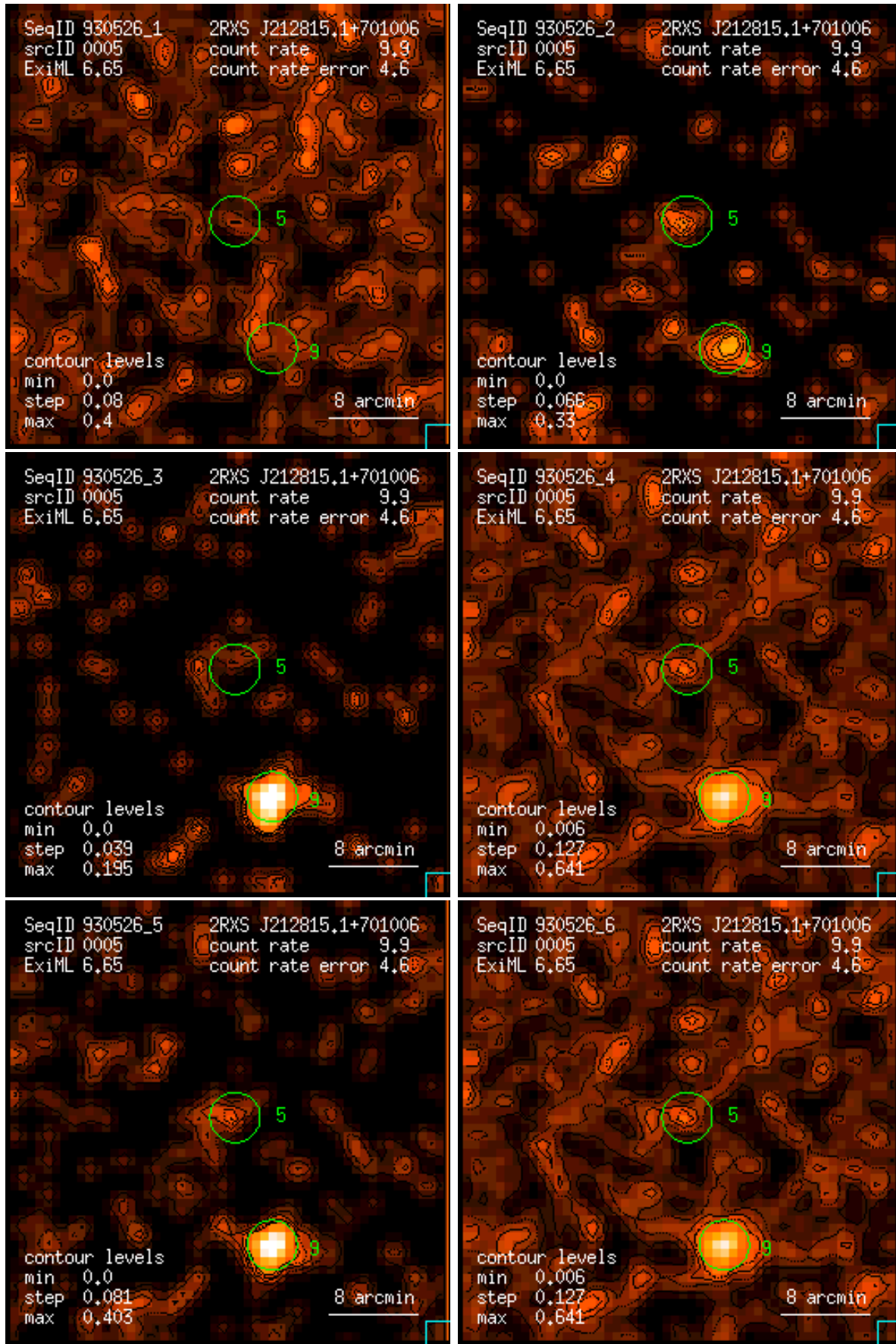
Figure 5: RASS 930526: detection 0005: band rate images, Gaussian filter: (1) PSPC channels 11 – 41, (2) 52 – 90, (3) 91 – 201, (4) 11 – 235, (5) 52 – 201, (6) 11 – 201. Broad band rates in counts/ks. Band rate contour levels in counts/ks/arcmin 2 .
