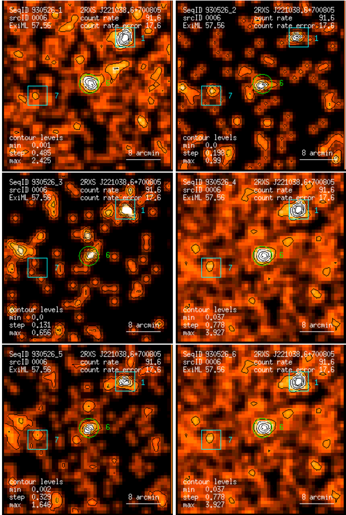
Figure 6: RASS 930526: detection 0006: band rate images, Gaussian filter: (1) PSPC channels 11 – 41, (2) 52 – 90, (3) 91 – 201, (4) 11 – 235, (5) 52 – 201, (6) 11 – 201. Broad band rates in counts/ks. Band rate contour levels in counts/ks/arcmin 2 .
