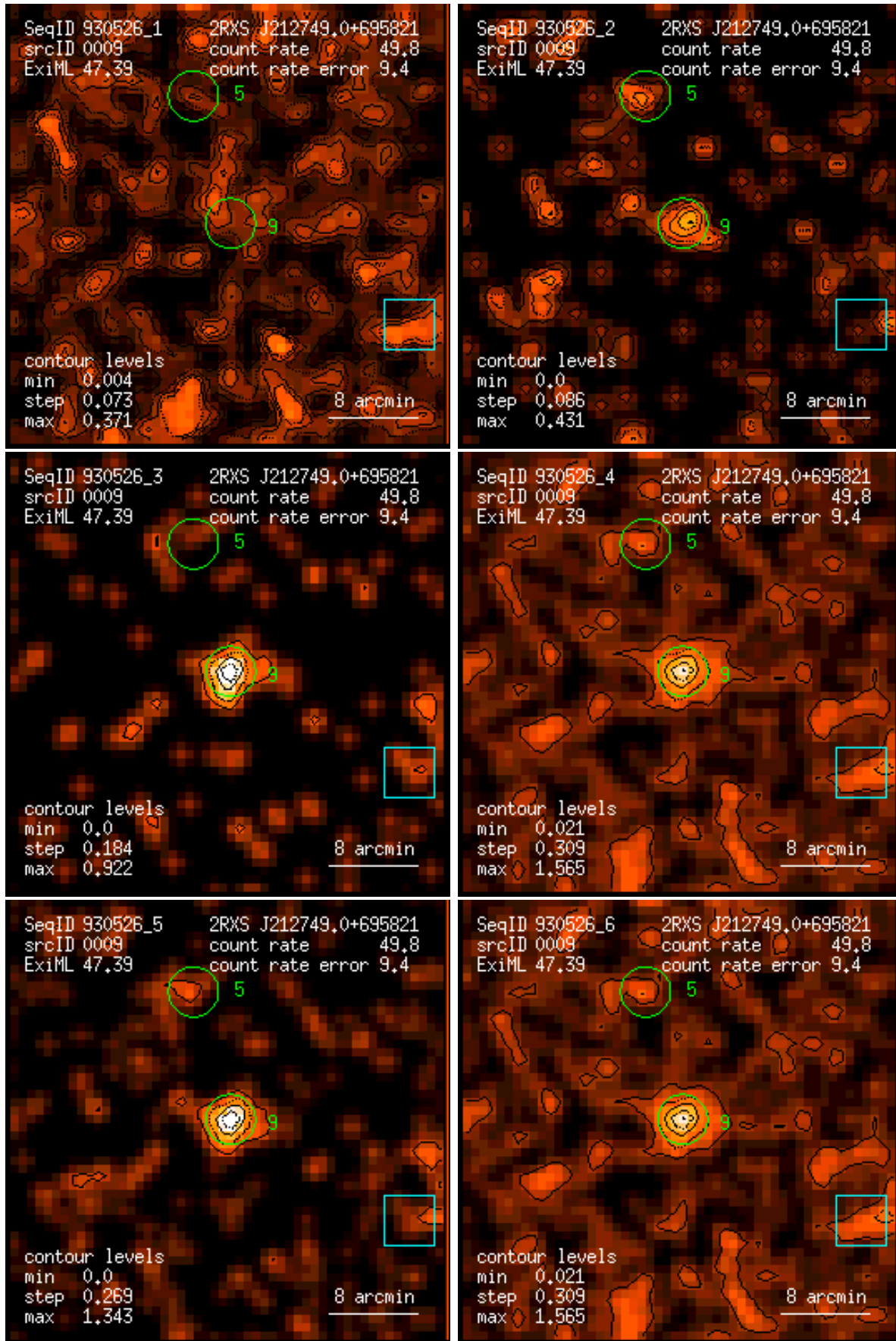
Figure 9: RASS 930526: detection 0009: band rate images, Gaussian filter: (1) PSPC channels 11 – 41, (2) 52 – 90, (3) 91 – 201, (4) 11 – 235, (5) 52 – 201, (6) 11 – 201. Broad band rates in counts/ks. Band rate contour levels in counts/ks/arcmin 2 .
