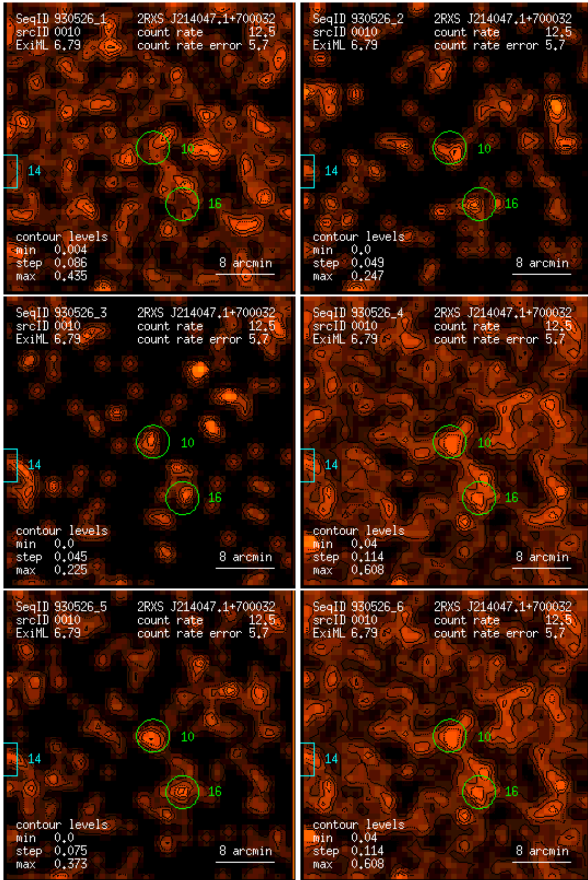
Figure 10: RASS 930526: detection 0010: band rate images, Gaussian filter: (1) PSPC channels 11 – 41, (2) 52 – 90, (3) 91 – 201, (4) 11 – 235, (5) 52 – 201, (6) 11 – 201. Broad band rates in counts/ks. Band rate contour levels in counts/ks/arcmin 2 .
