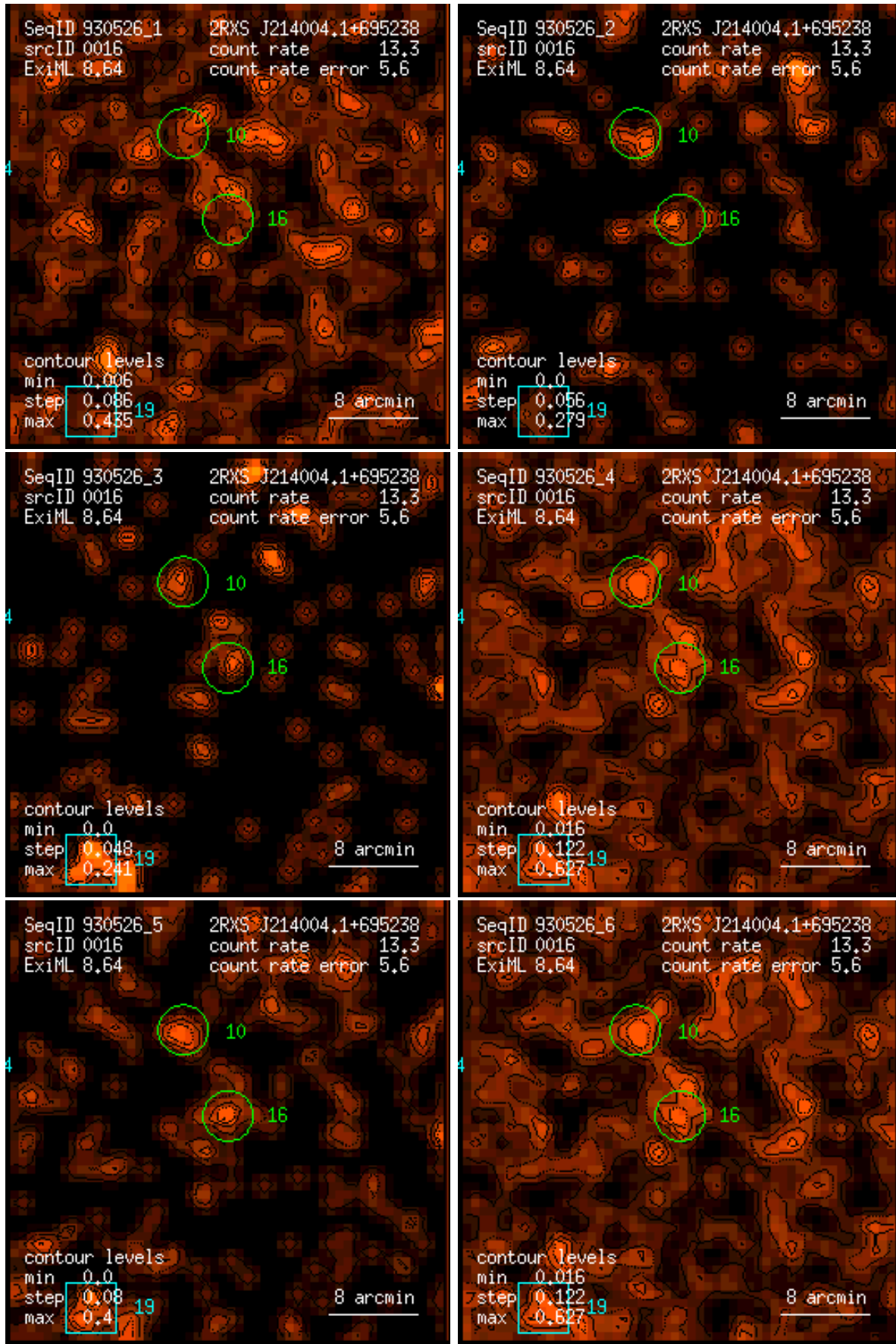
Figure 16: RASS 930526: detection 0016: band rate images, Gaussian filter: (1) PSPC channels 11 – 41, (2) 52 – 90, (3) 91 – 201, (4) 11 – 235, (5) 52 – 201, (6) 11 – 201. Broad band rates in counts/ks. Band rate contour levels in counts/ks/arcmin 2 .
