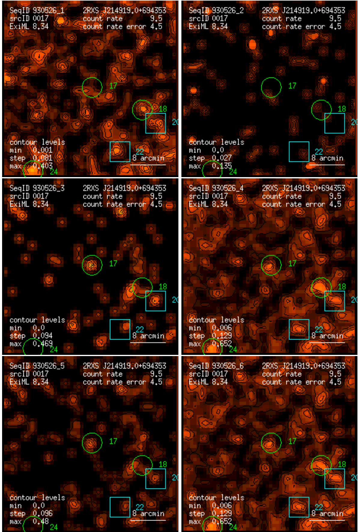
Figure 17: RASS 930526: detection 0017: band rate images, Gaussian filter: (1) PSPC channels 11 – 41, (2) 52 – 90, (3) 91 – 201, (4) 11 – 235, (5) 52 – 201, (6) 11 – 201. Broad band rates in counts/ks. Band rate contour levels in counts/ks/arcmin 2 .
