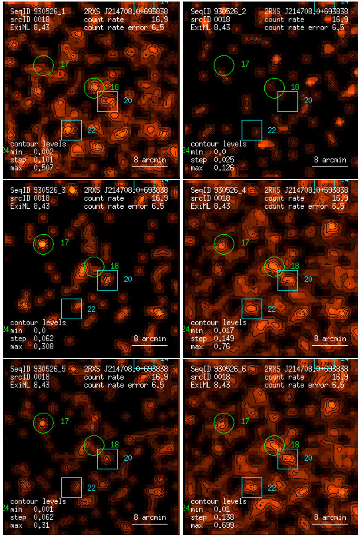
Figure 18: RASS 930526: detection 0018: band rate images, Gaussian filter: (1) PSPC channels 11 – 41, (2) 52 – 90, (3) 91 – 201, (4) 11 – 235, (5) 52 – 201, (6) 11 – 201. Broad band rates in counts/ks. Band rate contour levels in counts/ks/arcmin 2 .
