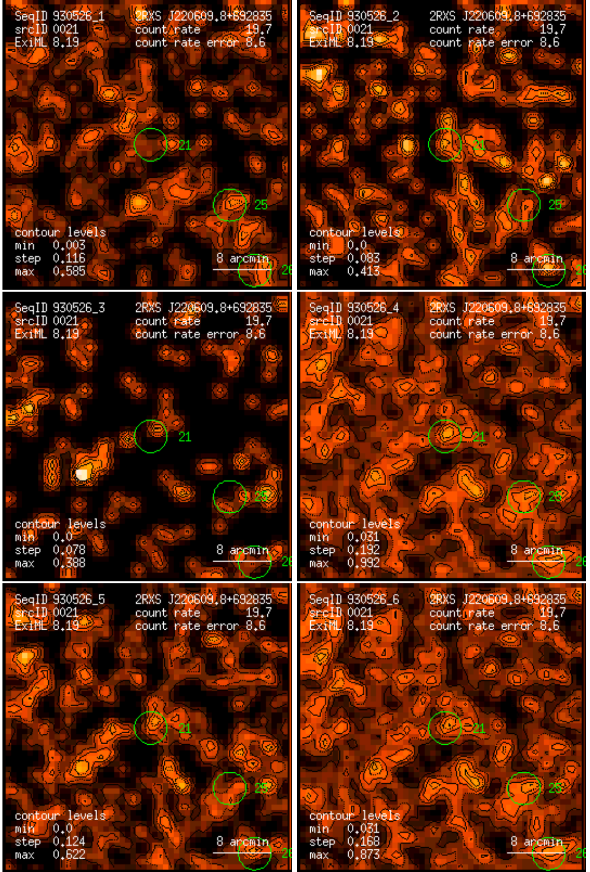
Figure 21: RASS 930526: detection 0021: band rate images, Gaussian filter: (1) PSPC channels 11 – 41, (2) 52 – 90, (3) 91 – 201, (4) 11 – 235, (5) 52 – 201, (6) 11 – 201. Broad band rates in counts/ks. Band rate contour levels in counts/ks/arcmin 2 .
