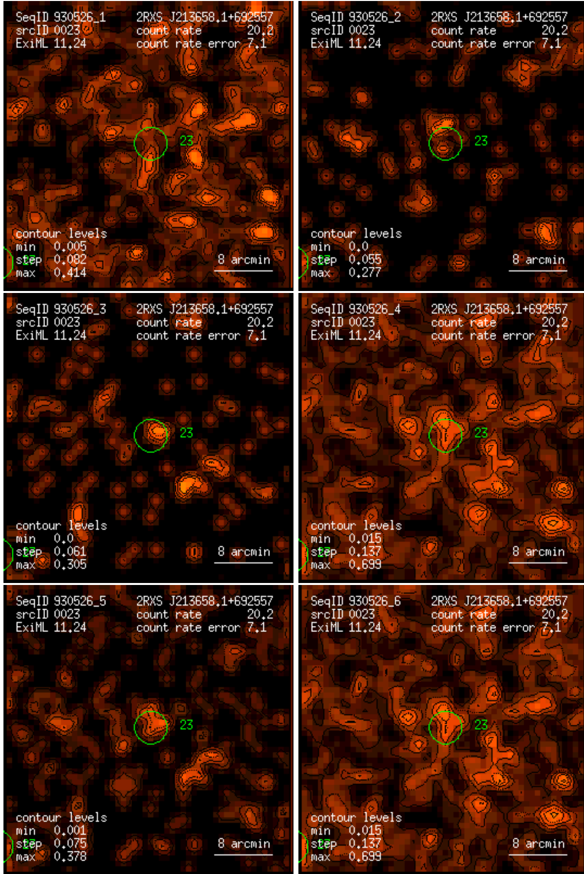
Figure 23: RASS 930526: detection 0023: band rate images, Gaussian filter: (1) PSPC channels 11 – 41, (2) 52 – 90, (3) 91 – 201, (4) 11 – 235, (5) 52 – 201, (6) 11 – 201. Broad band rates in counts/ks. Band rate contour levels in counts/ks/arcmin 2 .
