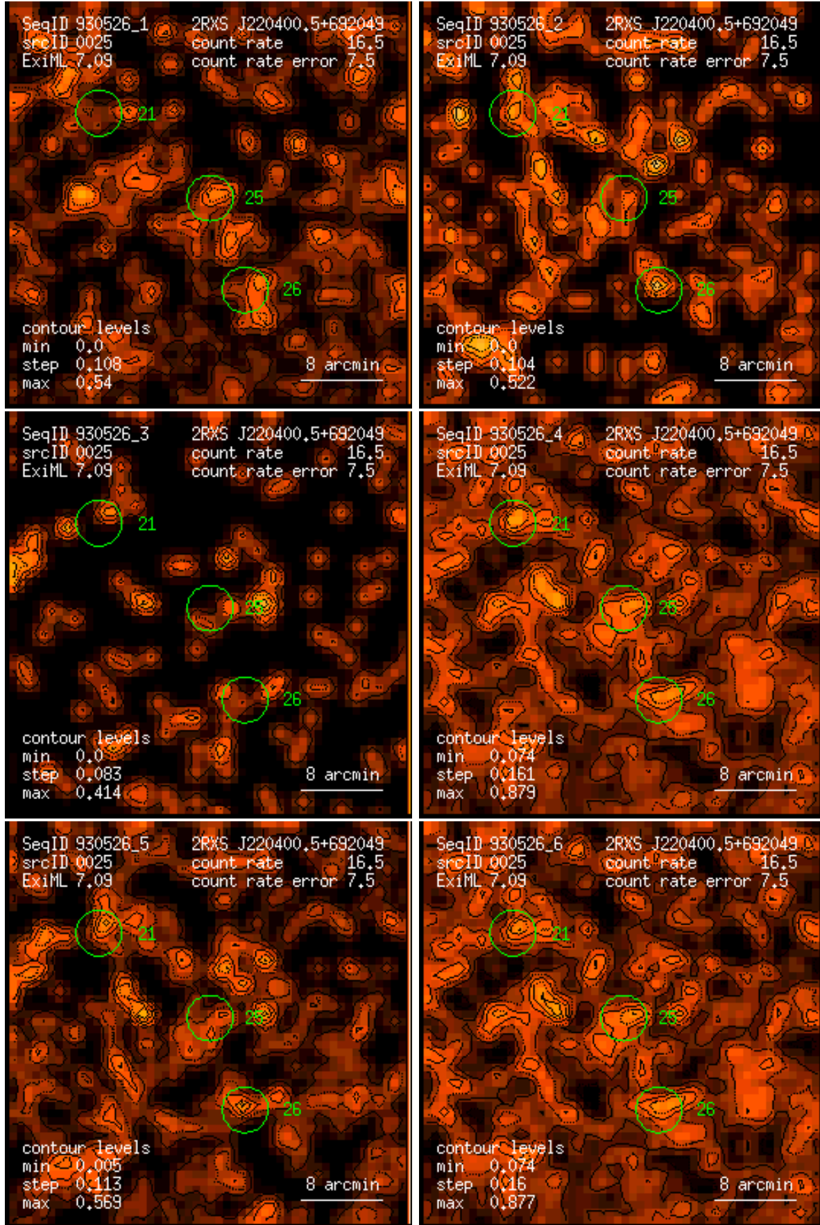
Figure 25: RASS 930526: detection 0025: band rate images, Gaussian filter: (1) PSPC channels 11 – 41, (2) 52 – 90, (3) 91 – 201, (4) 11 – 235, (5) 52 – 201, (6) 11 – 201. Broad band rates in counts/ks. Band rate contour levels in counts/ks/arcmin 2 .
