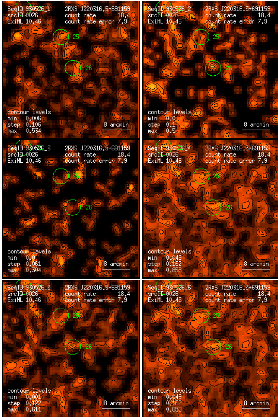
Figure 26: RASS 930526: detection 0026: band rate images, Gaussian filter: (1) PSPC channels 11 – 41, (2) 52 – 90, (3) 91 – 201, (4) 11 – 235, (5) 52 – 201, (6) 11 – 201. Broad band rates in counts/ks. Band rate contour levels in counts/ks/arcmin 2 .
