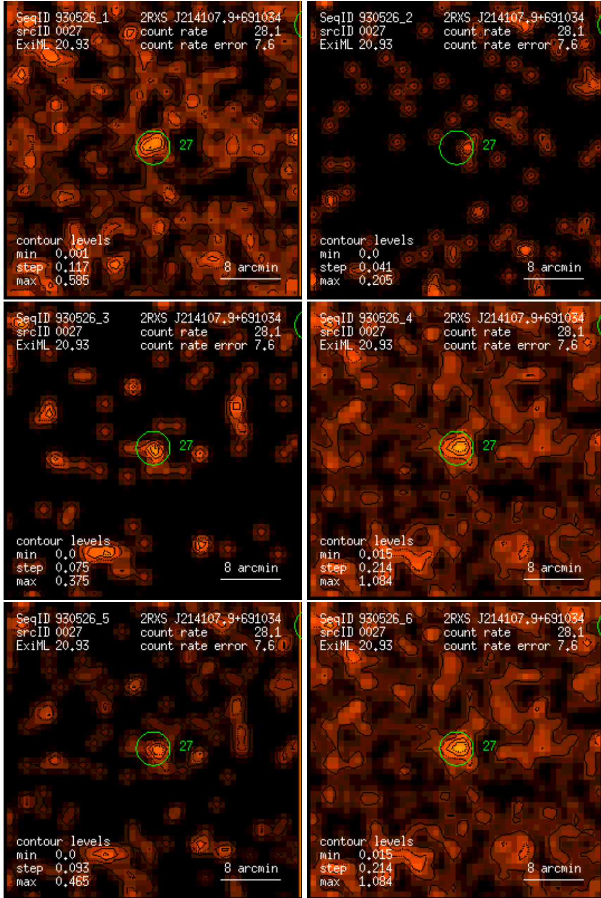
Figure 27: RASS 930526: detection 0027: band rate images, Gaussian filter: (1) PSPC channels 11 – 41, (2) 52 – 90, (3) 91 – 201, (4) 11 – 235, (5) 52 – 201, (6) 11 – 201. Broad band rates in counts/ks. Band rate contour levels in counts/ks/arcmin 2 .
