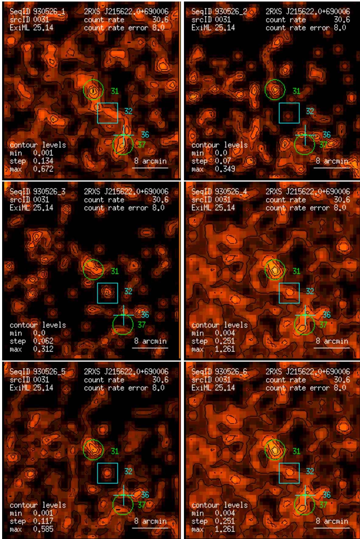
Figure 31: RASS 930526: detection 0031: band rate images, Gaussian filter: (1) PSPC channels 11 – 41, (2) 52 – 90, (3) 91 – 201, (4) 11 – 235, (5) 52 – 201, (6) 11 – 201. Broad band rates in counts/ks. Band rate contour levels in counts/ks/arcmin 2 .
