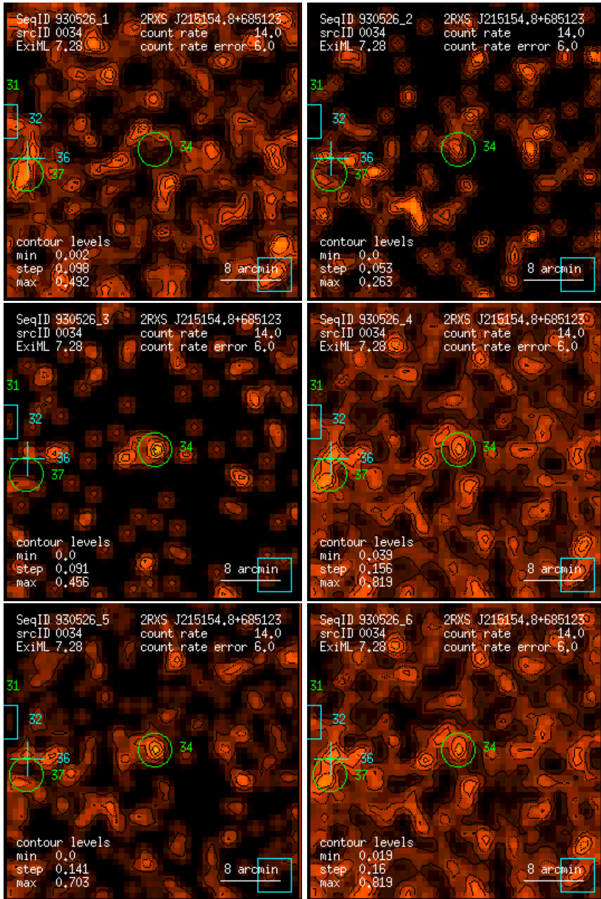
Figure 34: RASS 930526: detection 0034: band rate images, Gaussian filter: (1) PSPC channels 11 – 41, (2) 52 – 90, (3) 91 – 201, (4) 11 – 235, (5) 52 – 201, (6) 11 – 201. Broad band rates in counts/ks. Band rate contour levels in counts/ks/arcmin 2 .
