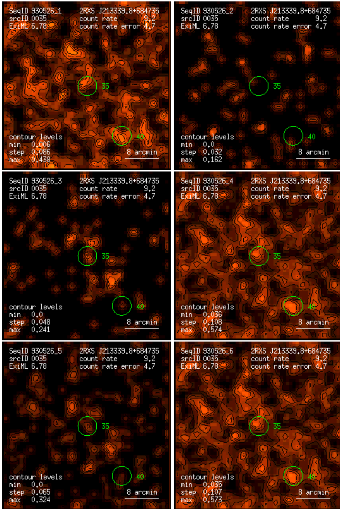
Figure 35: RASS 930526: detection 0035: band rate images, Gaussian filter: (1) PSPC channels 11 – 41, (2) 52 – 90, (3) 91 – 201, (4) 11 – 235, (5) 52 – 201, (6) 11 – 201. Broad band rates in counts/ks. Band rate contour levels in counts/ks/arcmin 2 .
