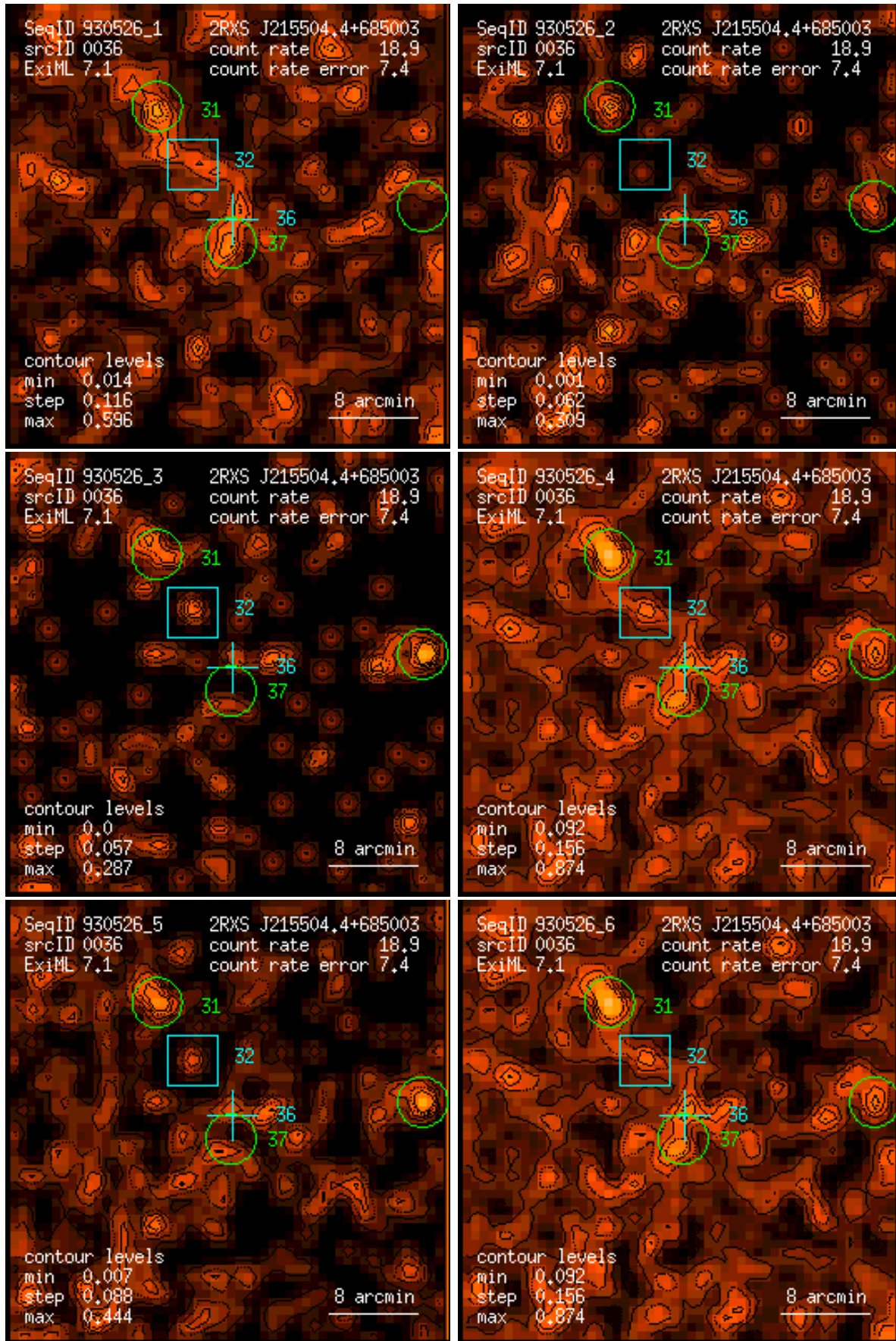
Figure 36: RASS 930526: detection 0036: band rate images, Gaussian filter: (1) PSPC channels 11 – 41, (2) 52 – 90, (3) 91 – 201, (4) 11 – 235, (5) 52 – 201, (6) 11 – 201. Broad band rates in counts/ks. Band rate contour levels in counts/ks/arcmin 2 .
