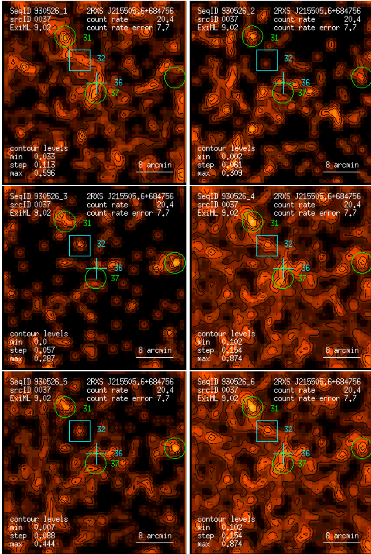
Figure 37: RASS 930526: detection 0037: band rate images, Gaussian filter: (1) PSPC channels 11 – 41, (2) 52 – 90, (3) 91 – 201, (4) 11 – 235, (5) 52 – 201, (6) 11 – 201. Broad band rates in counts/ks. Band rate contour levels in counts/ks/arcmin 2 .
