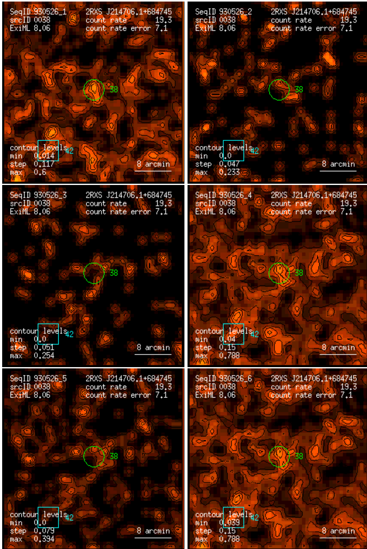
Figure 38: RASS 930526: detection 0038: band rate images, Gaussian filter: (1) PSPC channels 11 – 41, (2) 52 – 90, (3) 91 – 201, (4) 11 – 235, (5) 52 – 201, (6) 11 – 201. Broad band rates in counts/ks. Band rate contour levels in counts/ks/arcmin 2 .
