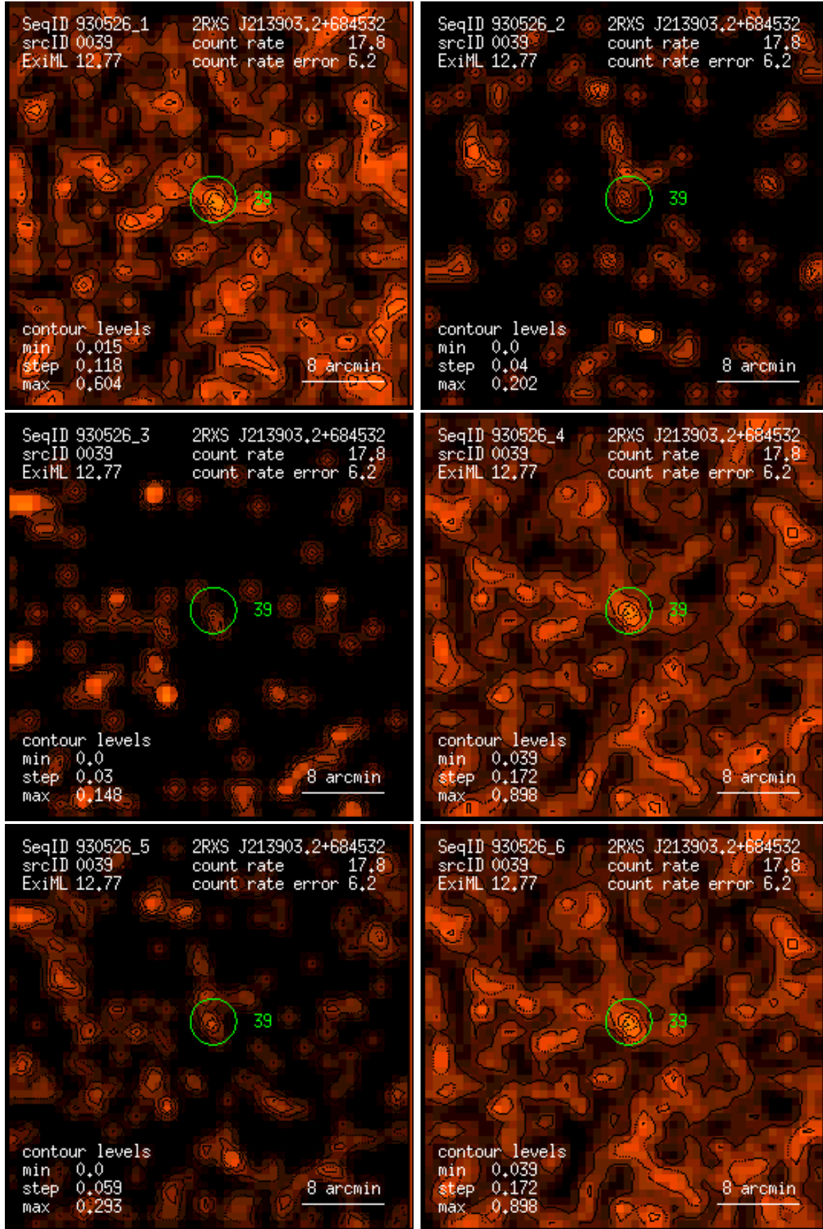
Figure 39: RASS 930526: detection 0039: band rate images, Gaussian filter: (1) PSPC channels 11 – 41, (2) 52 – 90, (3) 91 – 201, (4) 11 – 235, (5) 52 – 201, (6) 11 – 201. Broad band rates in counts/ks. Band rate contour levels in counts/ks/arcmin 2 .
