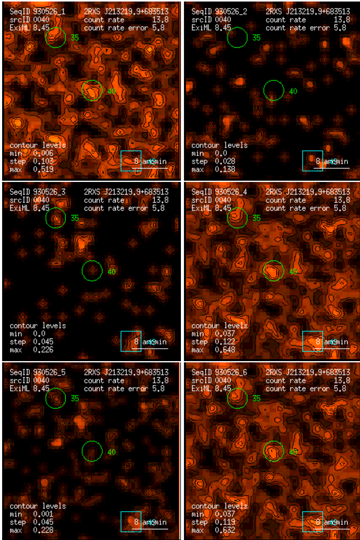
Figure 40: RASS 930526: detection 0040: band rate images, Gaussian filter: (1) PSPC channels 11 – 41, (2) 52 – 90, (3) 91 – 201, (4) 11 – 235, (5) 52 – 201, (6) 11 – 201. Broad band rates in counts/ks. Band rate contour levels in counts/ks/arcmin 2 .
