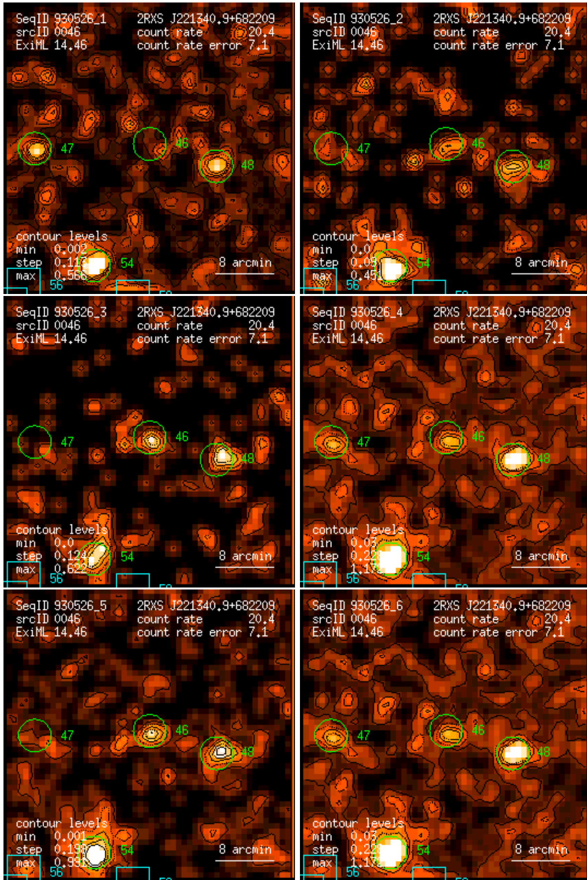
Figure 46: RASS 930526: detection 0046: band rate images, Gaussian filter: (1) PSPC channels 11 – 41, (2) 52 – 90, (3) 91 – 201, (4) 11 – 235, (5) 52 – 201, (6) 11 – 201. Broad band rates in counts/ks. Band rate contour levels in counts/ks/arcmin 2 .
