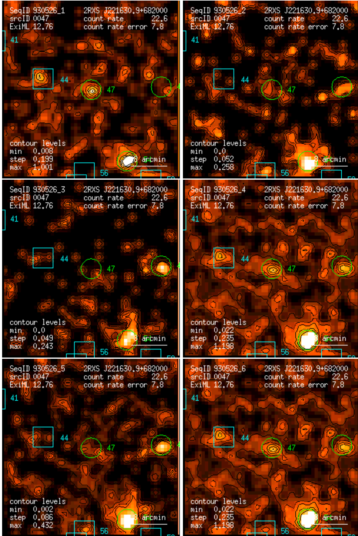
Figure 47: RASS 930526: detection 0047: band rate images, Gaussian filter: (1) PSPC channels 11 – 41, (2) 52 – 90, (3) 91 – 201, (4) 11 – 235, (5) 52 – 201, (6) 11 – 201. Broad band rates in counts/ks. Band rate contour levels in counts/ks/arcmin 2 .
