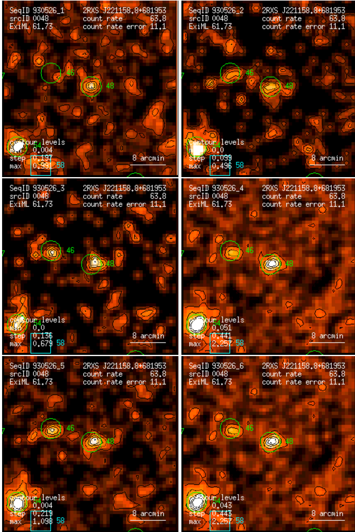
Figure 48: RASS 930526: detection 0048: band rate images, Gaussian filter: (1) PSPC channels 11 – 41, (2) 52 – 90, (3) 91 – 201, (4) 11 – 235, (5) 52 – 201, (6) 11 – 201. Broad band rates in counts/ks. Band rate contour levels in counts/ks/arcmin 2 .
