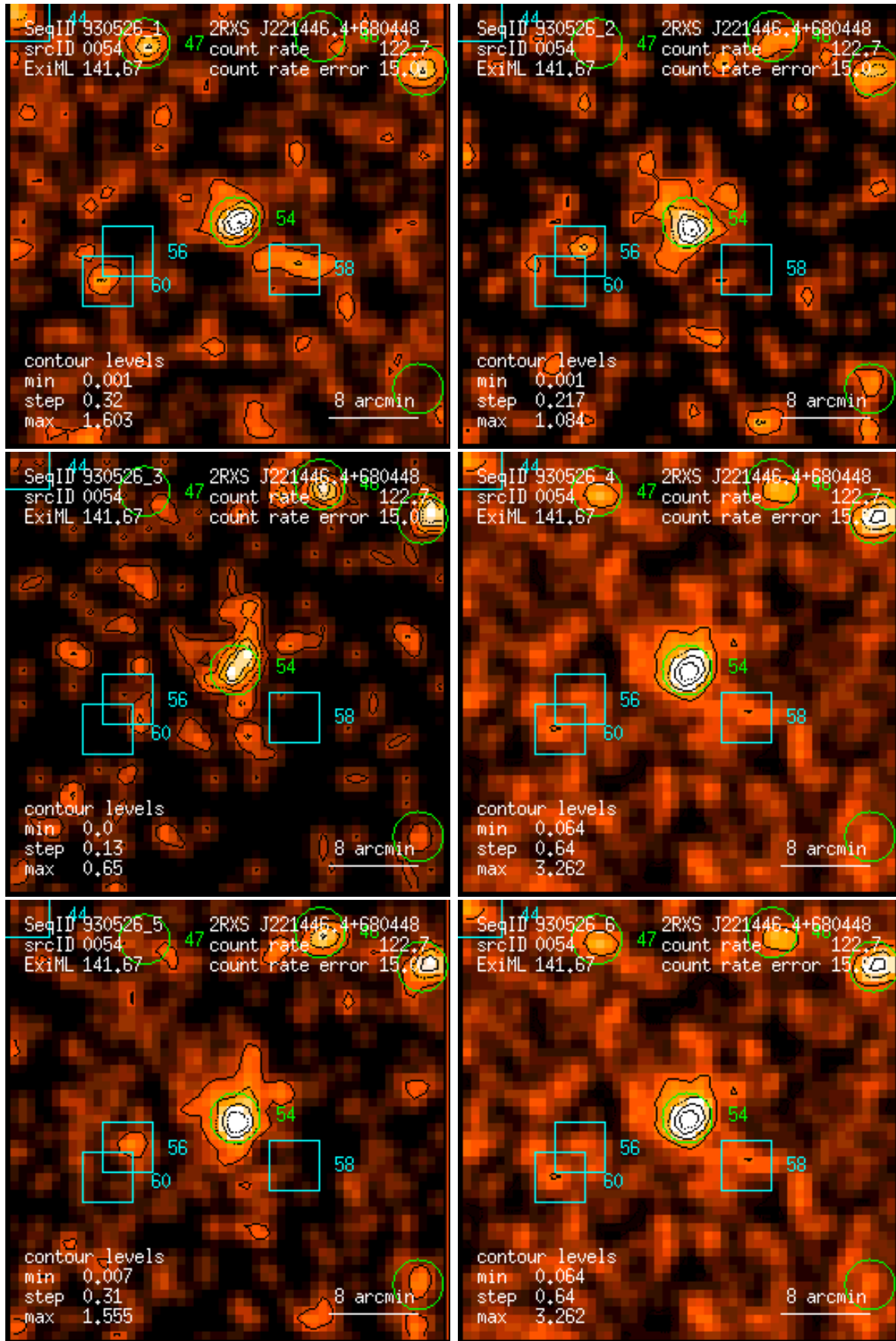
Figure 54: RASS 930526: detection 0054: band rate images, Gaussian filter: (1) PSPC channels 11 – 41, (2) 52 – 90, (3) 91 – 201, (4) 11 – 235, (5) 52 – 201, (6) 11 – 201. Broad band rates in counts/ks. Band rate contour levels in counts/ks/arcmin 2 .
