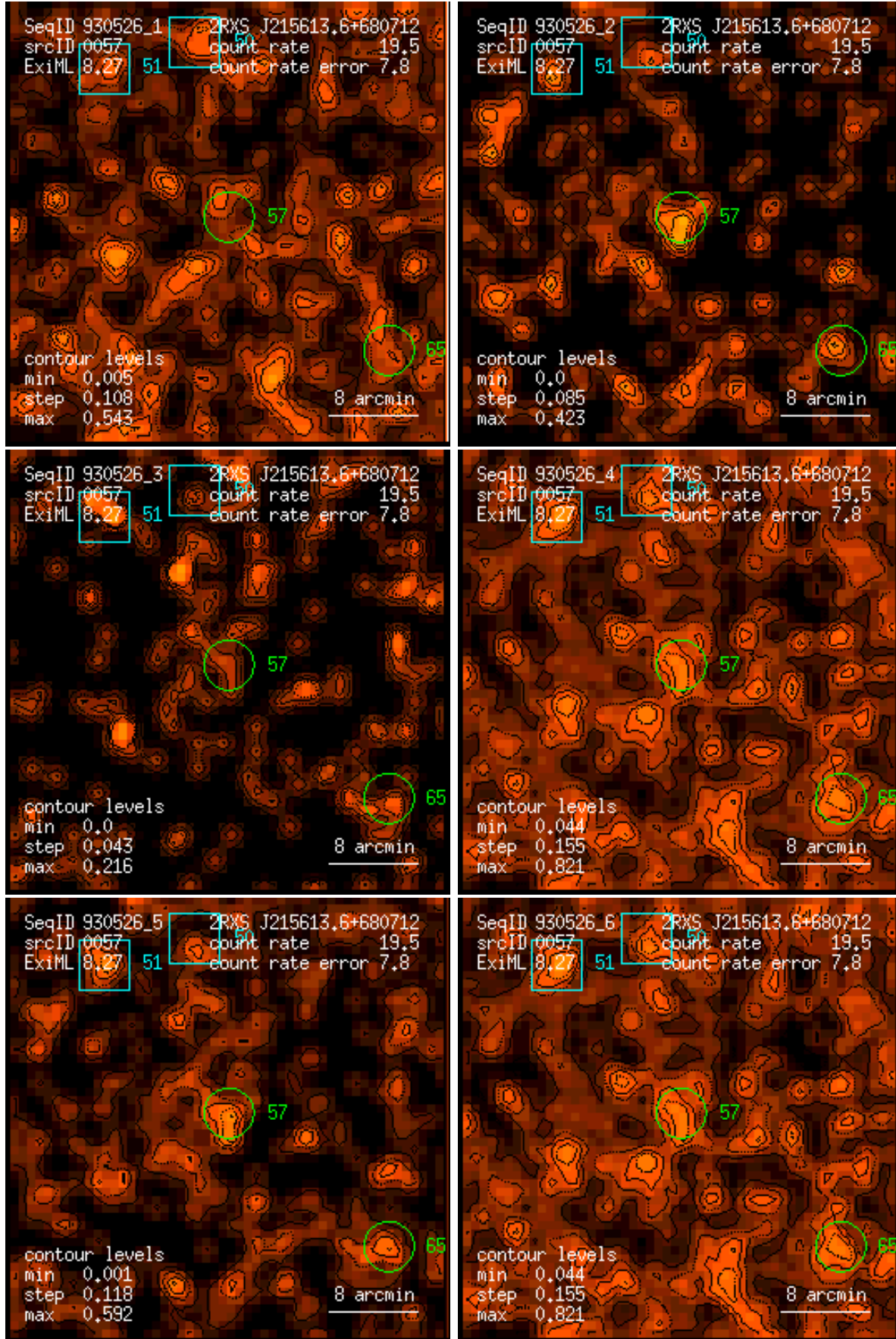
Figure 57: RASS 930526: detection 0057: band rate images, Gaussian filter: (1) PSPC channels 11 – 41, (2) 52 – 90, (3) 91 – 201, (4) 11 – 235, (5) 52 – 201, (6) 11 – 201. Broad band rates in counts/ks. Band rate contour levels in counts/ks/arcmin 2 .
