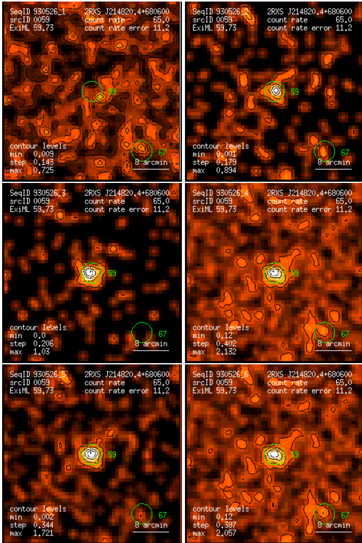
Figure 59: RASS 930526: detection 0059: band rate images, Gaussian filter: (1) PSPC channels 11 – 41, (2) 52 – 90, (3) 91 – 201, (4) 11 – 235, (5) 52 – 201, (6) 11 – 201. Broad band rates in counts/ks. Band rate contour levels in counts/ks/arcmin 2 .
