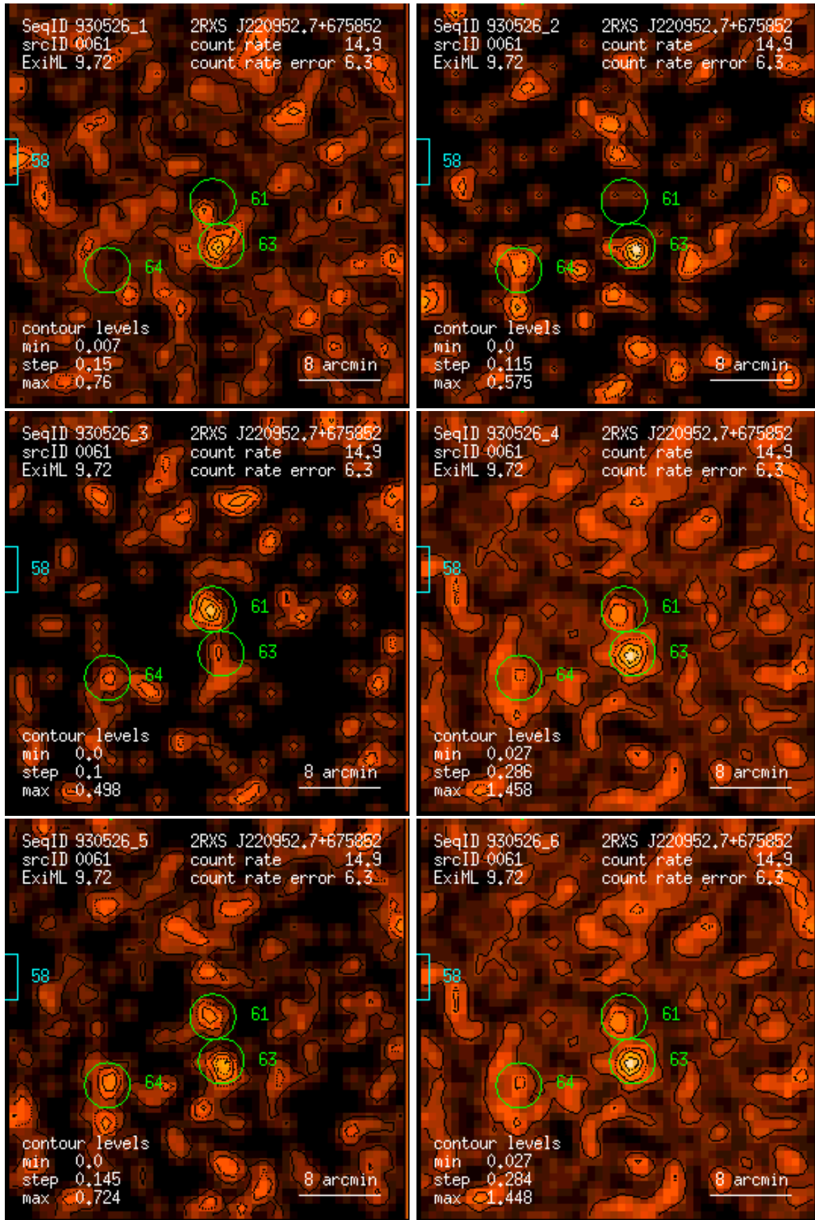
Figure 61: RASS 930526: detection 0061: band rate images, Gaussian filter: (1) PSPC channels 11 – 41, (2) 52 – 90, (3) 91 – 201, (4) 11 – 235, (5) 52 – 201, (6) 11 – 201. Broad band rates in counts/ks. Band rate contour levels in counts/ks/arcmin 2 .
