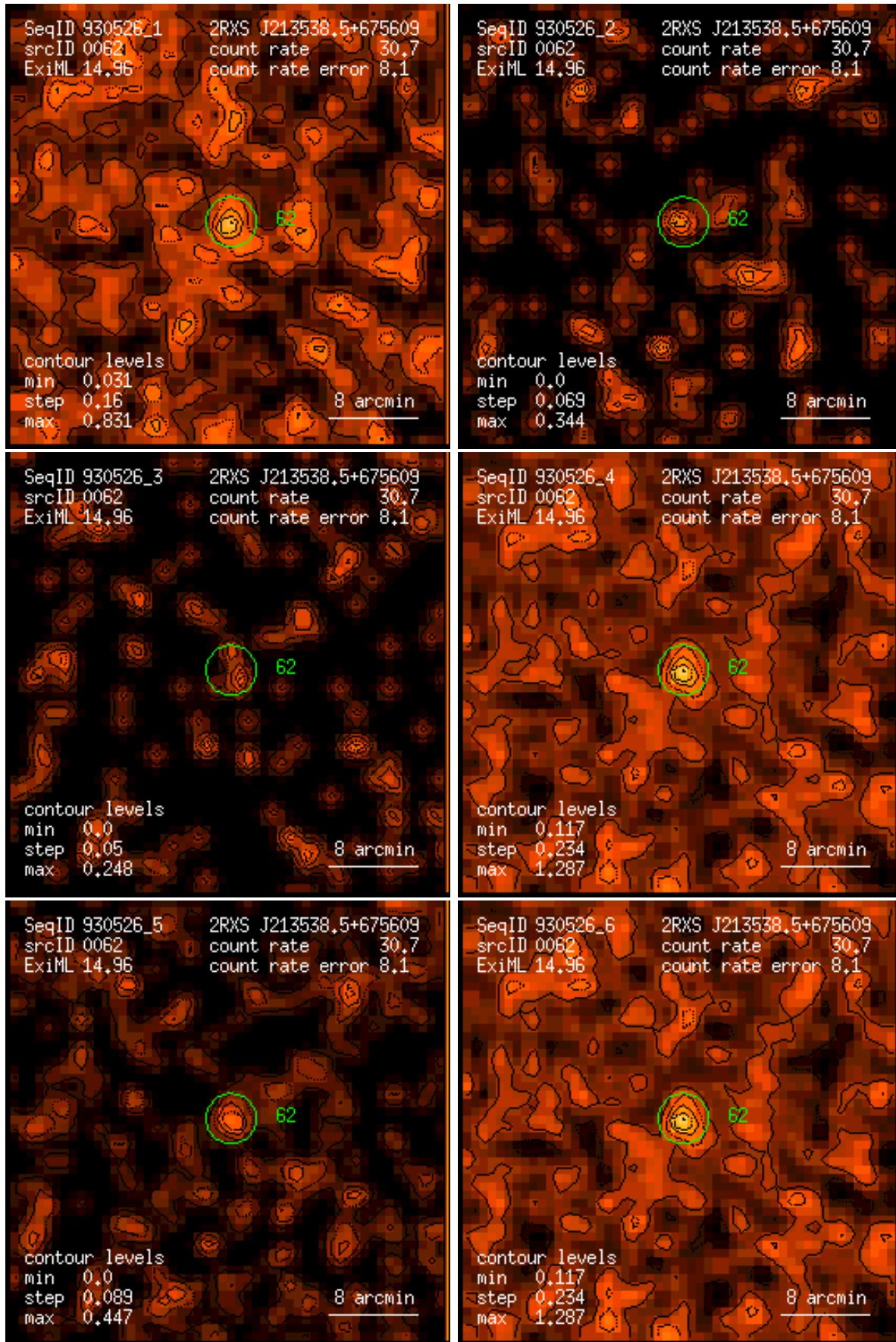
Figure 62: RASS 930526: detection 0062: band rate images, Gaussian filter: (1) PSPC channels 11 – 41, (2) 52 – 90, (3) 91 – 201, (4) 11 – 235, (5) 52 – 201, (6) 11 – 201. Broad band rates in counts/ks. Band rate contour levels in counts/ks/arcmin 2 .
