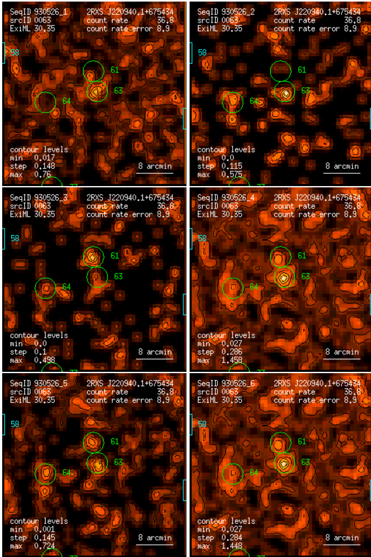
Figure 63: RASS 930526: detection 0063: band rate images, Gaussian filter: (1) PSPC channels 11 – 41, (2) 52 – 90, (3) 91 – 201, (4) 11 – 235, (5) 52 – 201, (6) 11 – 201. Broad band rates in counts/ks. Band rate contour levels in counts/ks/arcmin 2 .
