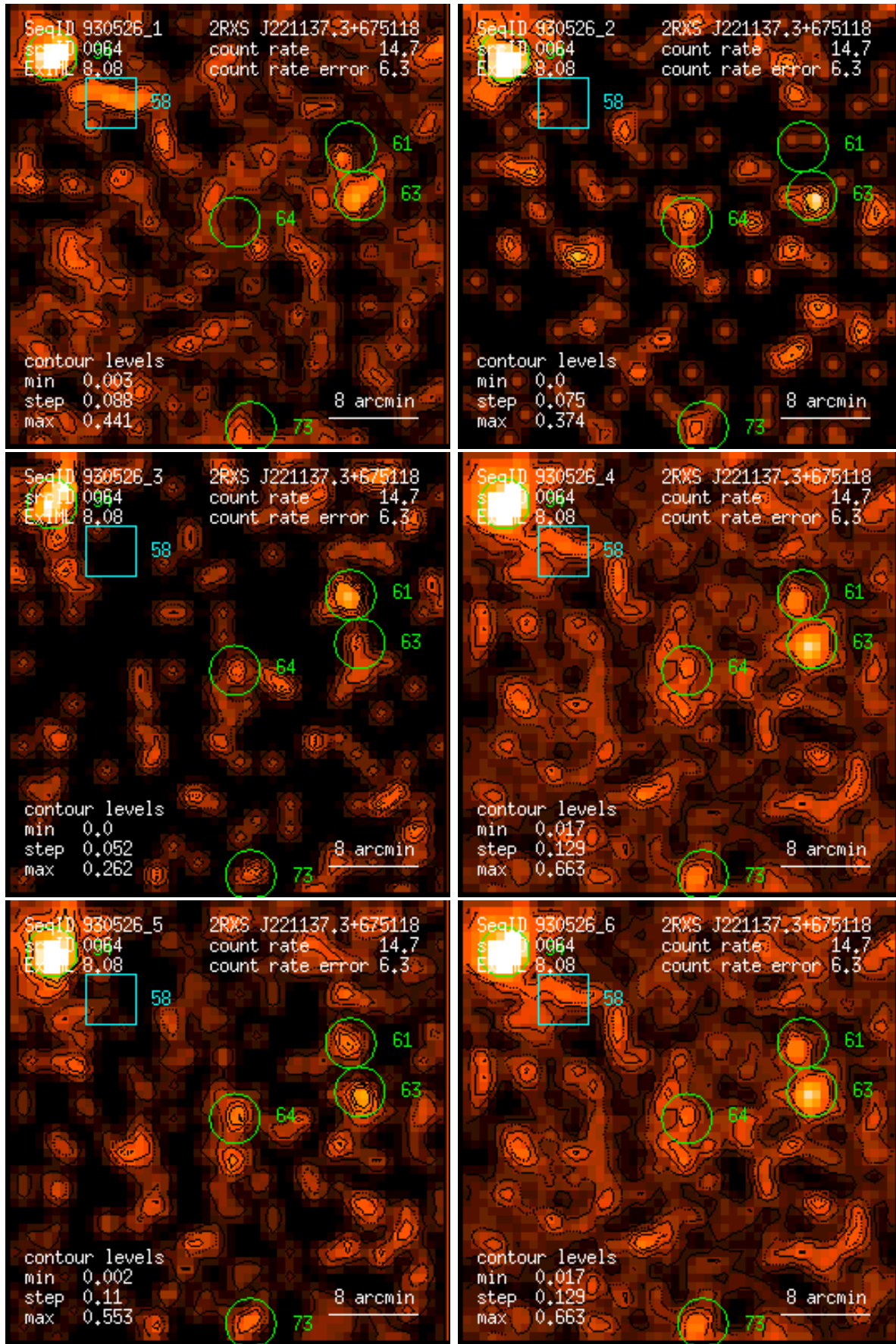
Figure 64: RASS 930526: detection 0064: band rate images, Gaussian filter: (1) PSPC channels 11 – 41, (2) 52 – 90, (3) 91 – 201, (4) 11 – 235, (5) 52 – 201, (6) 11 – 201. Broad band rates in counts/ks. Band rate contour levels in counts/ks/arcmin 2 .
