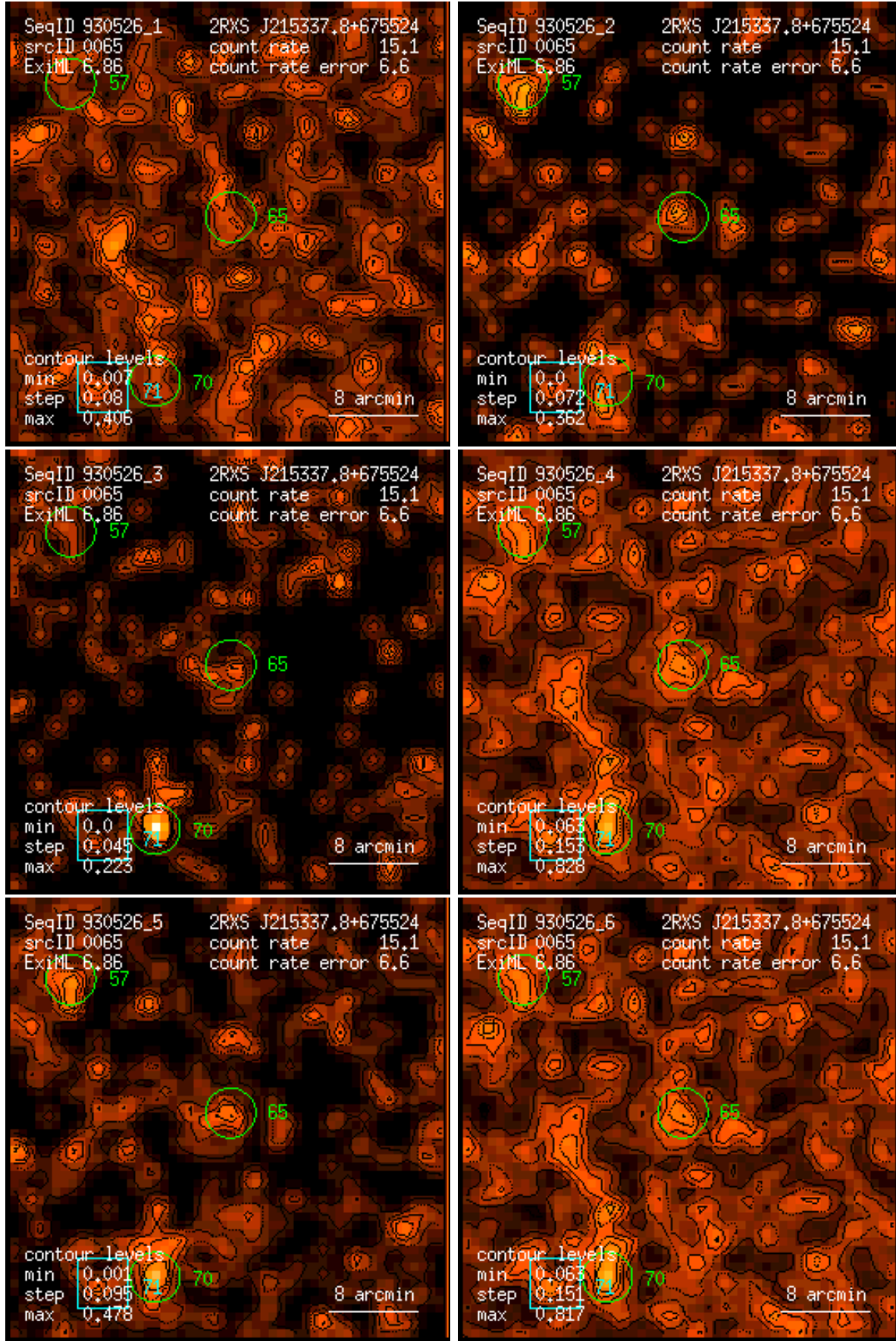
Figure 65: RASS 930526: detection 0065: band rate images, Gaussian filter: (1) PSPC channels 11 – 41, (2) 52 – 90, (3) 91 – 201, (4) 11 – 235, (5) 52 – 201, (6) 11 – 201. Broad band rates in counts/ks. Band rate contour levels in counts/ks/arcmin 2 .
