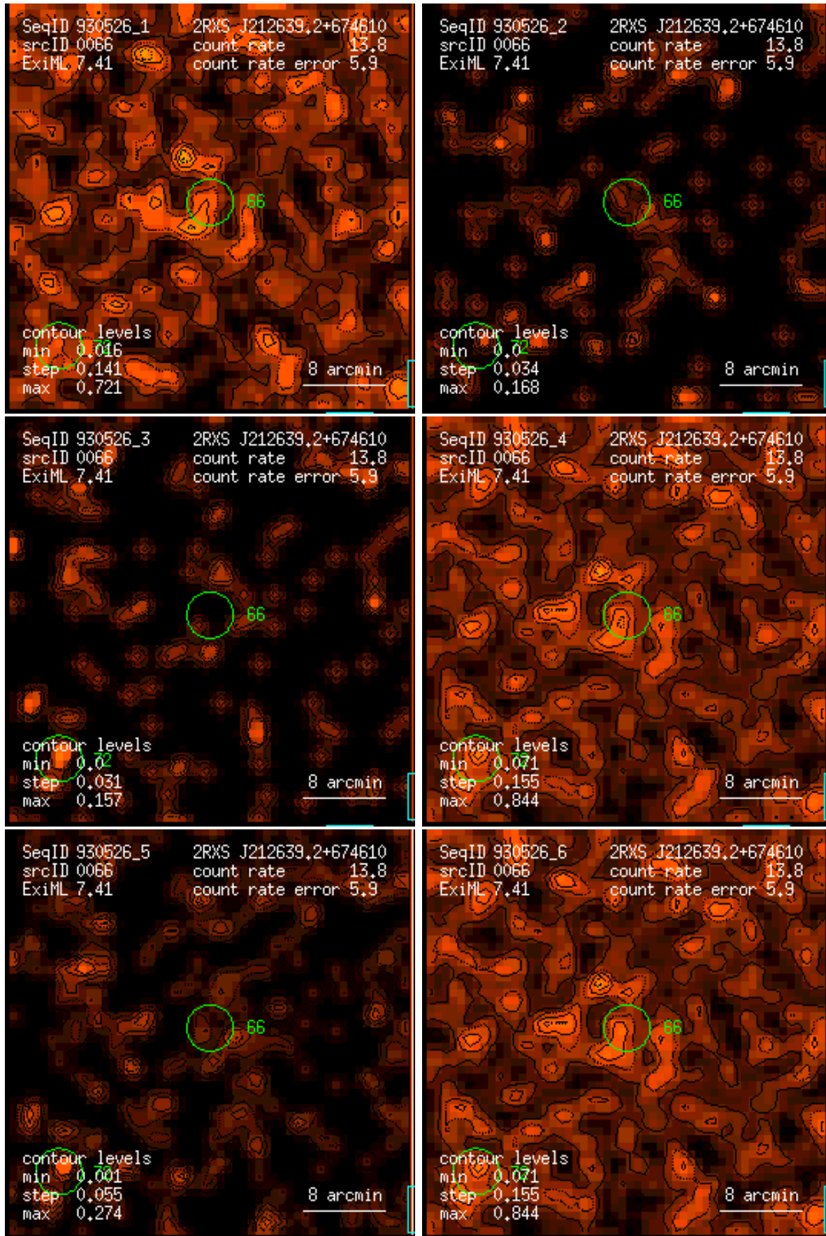
Figure 66: RASS 930526: detection 0066: band rate images, Gaussian filter: (1) PSPC channels 11 – 41, (2) 52 – 90, (3) 91 – 201, (4) 11 – 235, (5) 52 – 201, (6) 11 – 201. Broad band rates in counts/ks. Band rate contour levels in counts/ks/arcmin 2 .
