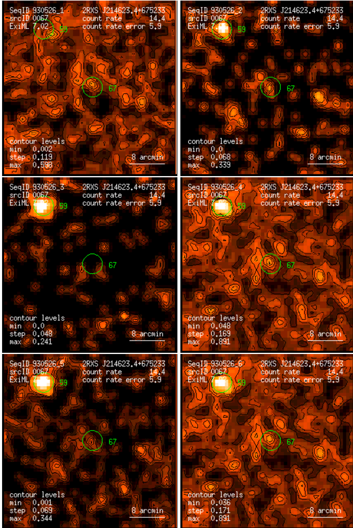
Figure 67: RASS 930526: detection 0067: band rate images, Gaussian filter: (1) PSPC channels 11 – 41, (2) 52 – 90, (3) 91 – 201, (4) 11 – 235, (5) 52 – 201, (6) 11 – 201. Broad band rates in counts/ks. Band rate contour levels in counts/ks/arcmin 2 .
