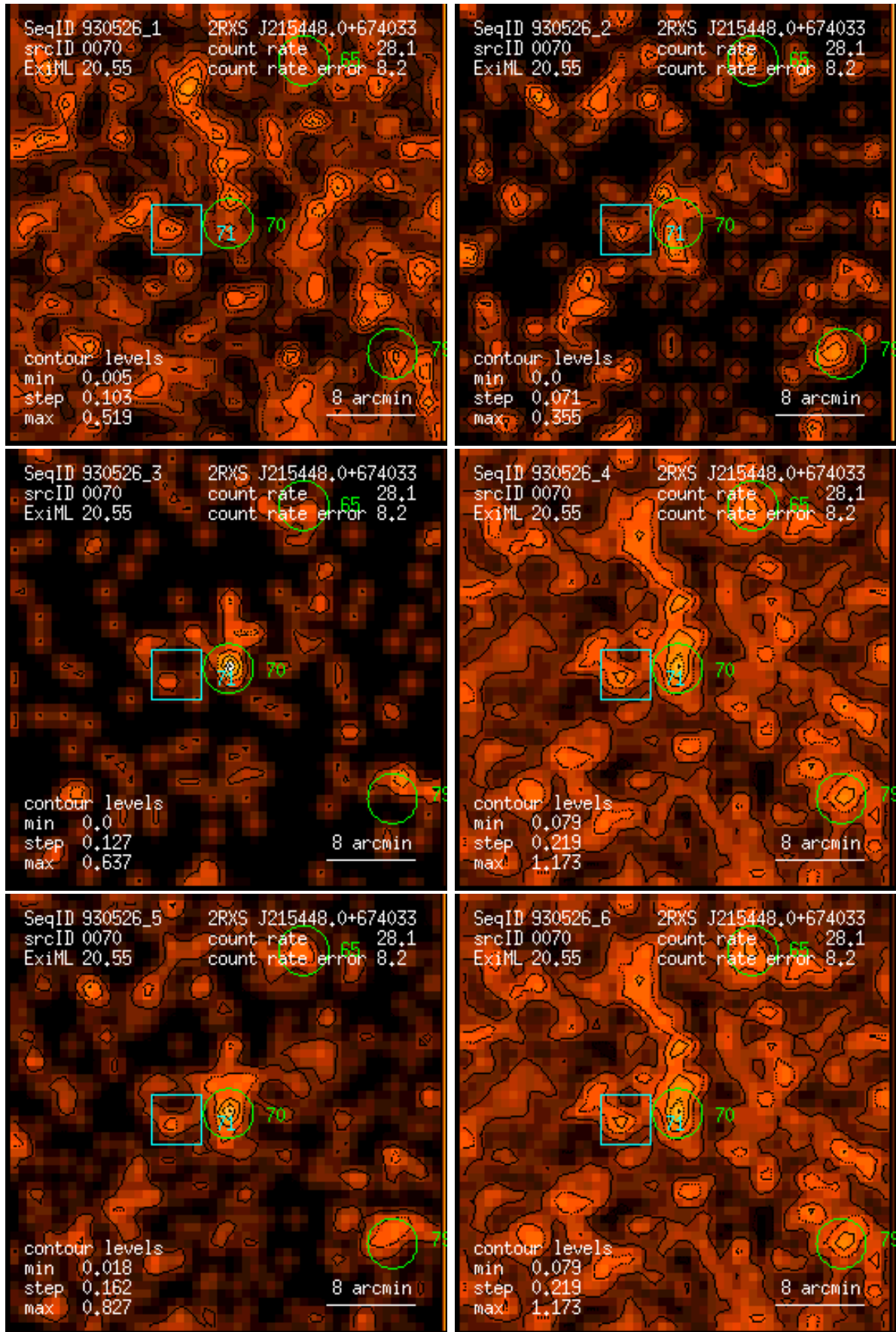
Figure 70: RASS 930526: detection 0070: band rate images, Gaussian filter: (1) PSPC channels 11 – 41, (2) 52 – 90, (3) 91 – 201, (4) 11 – 235, (5) 52 – 201, (6) 11 – 201. Broad band rates in counts/ks. Band rate contour levels in counts/ks/arcmin 2 .
