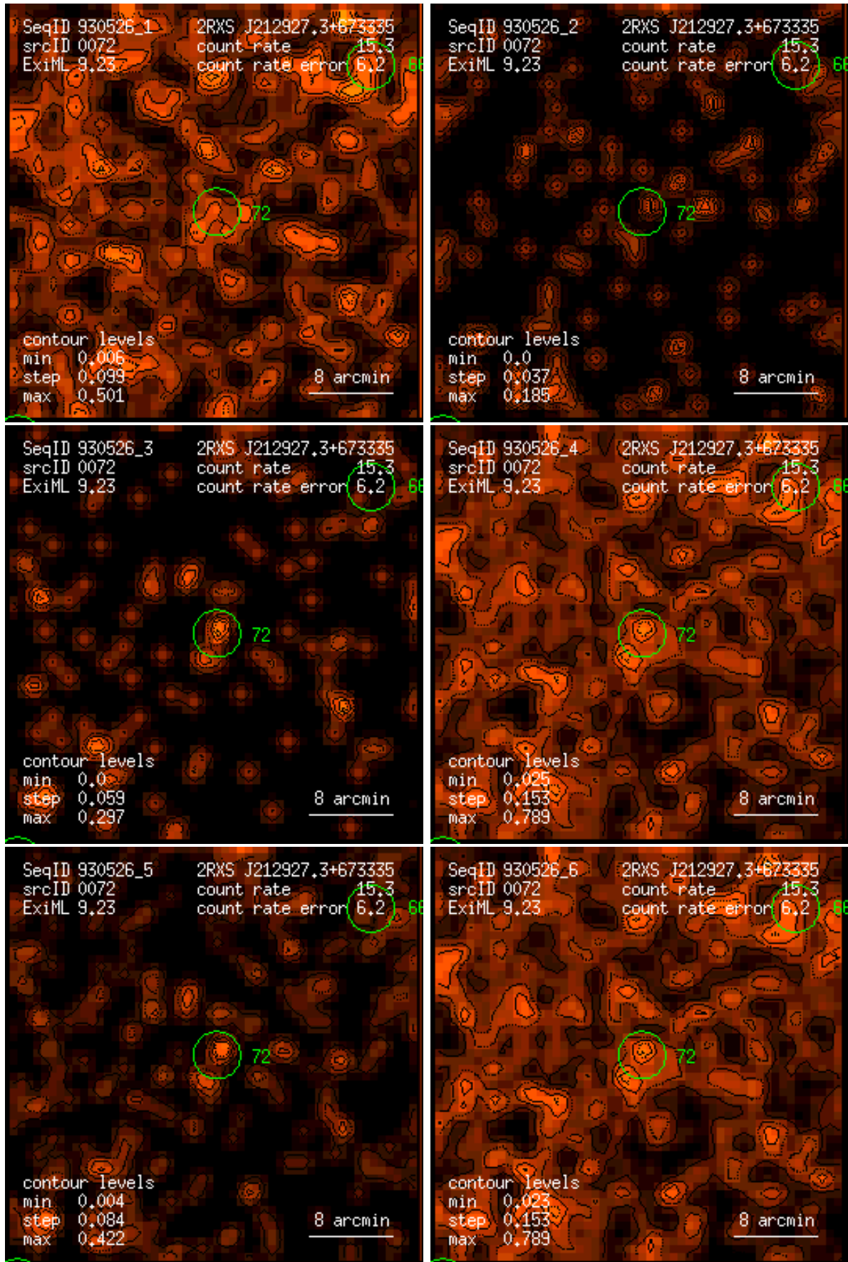
Figure 72: RASS 930526: detection 0072: band rate images, Gaussian filter: (1) PSPC channels 11 – 41, (2) 52 – 90, (3) 91 – 201, (4) 11 – 235, (5) 52 – 201, (6) 11 – 201. Broad band rates in counts/ks. Band rate contour levels in counts/ks/arcmin 2 .
