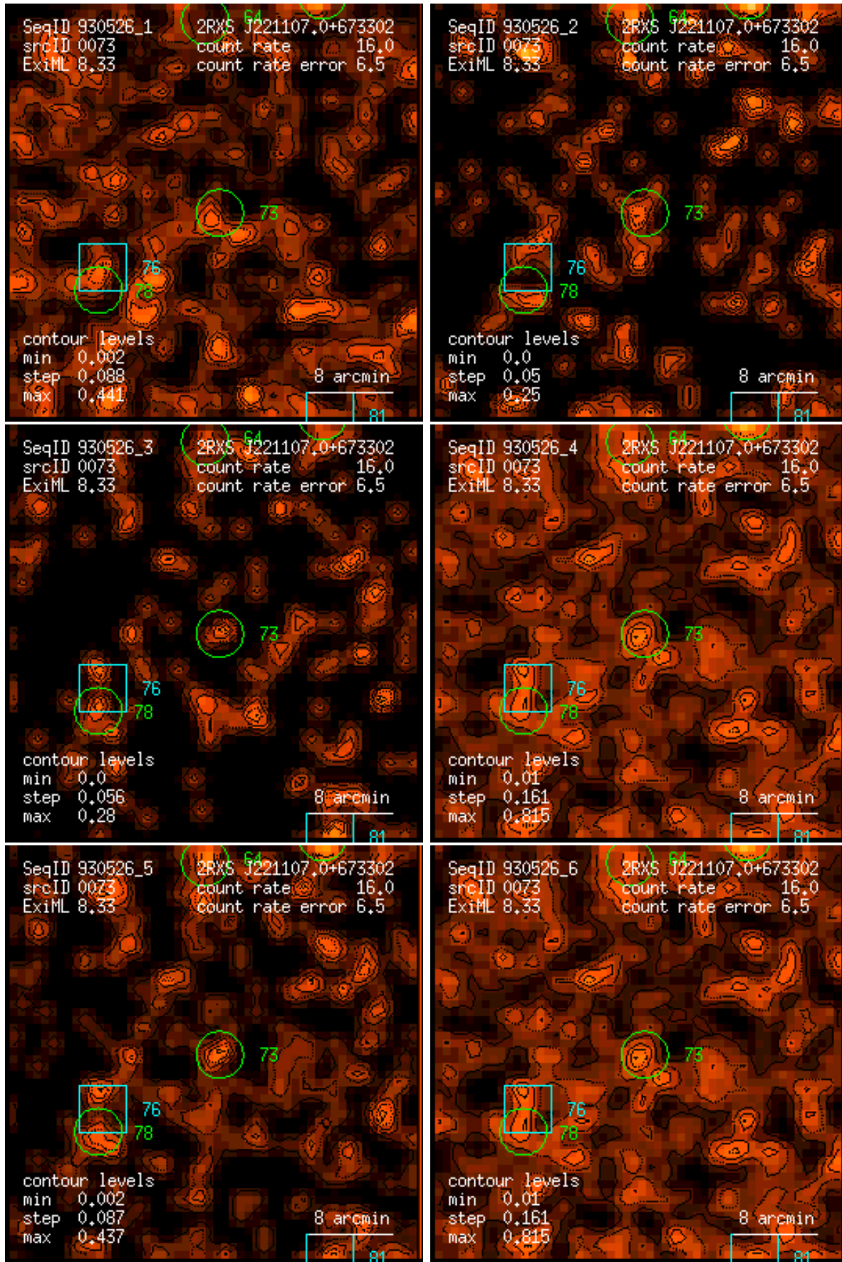
Figure 73: RASS 930526: detection 0073: band rate images, Gaussian filter: (1) PSPC channels 11 – 41, (2) 52 – 90, (3) 91 – 201, (4) 11 – 235, (5) 52 – 201, (6) 11 – 201. Broad band rates in counts/ks. Band rate contour levels in counts/ks/arcmin 2 .
