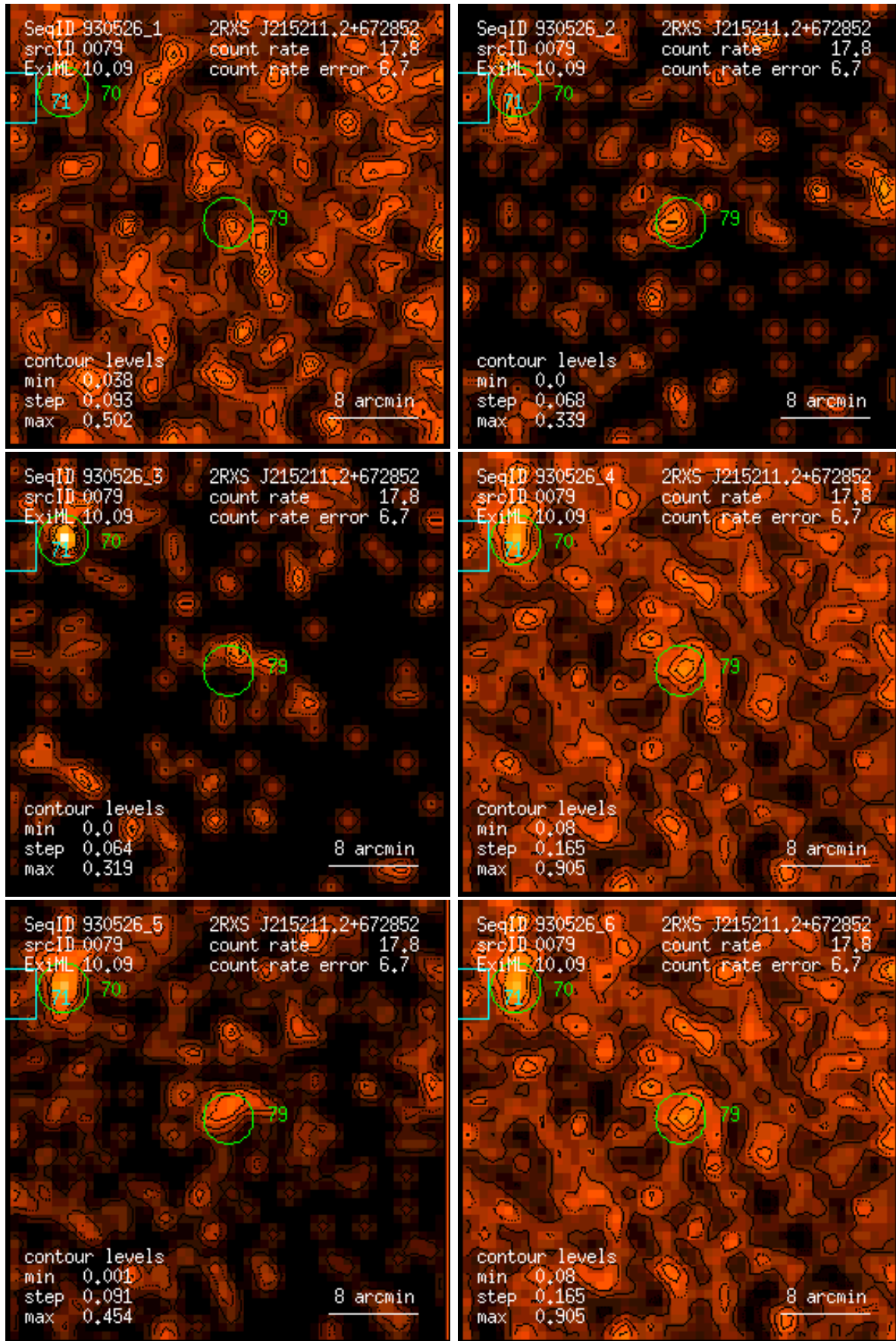
Figure 79: RASS 930526: detection 0079: band rate images, Gaussian filter: (1) PSPC channels 11 – 41, (2) 52 – 90, (3) 91 – 201, (4) 11 – 235, (5) 52 – 201, (6) 11 – 201. Broad band rates in counts/ks. Band rate contour levels in counts/ks/arcmin 2 .
