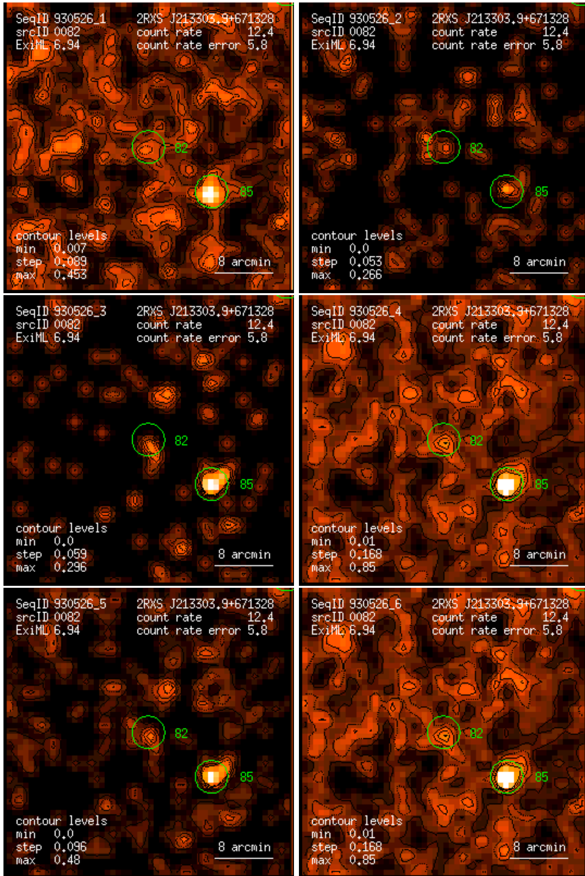
Figure 82: RASS 930526: detection 0082: band rate images, Gaussian filter: (1) PSPC channels 11 – 41, (2) 52 – 90, (3) 91 – 201, (4) 11 – 235, (5) 52 – 201, (6) 11 – 201. Broad band rates in counts/ks. Band rate contour levels in counts/ks/arcmin 2 .
