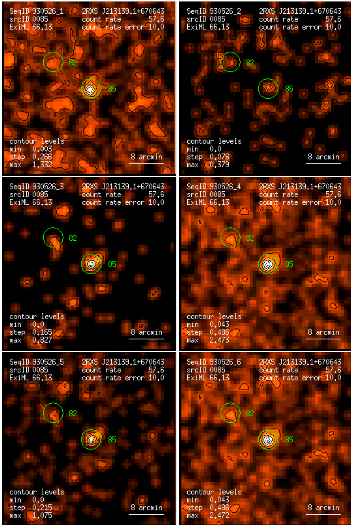
Figure 85: RASS 930526: detection 0085: band rate images, Gaussian filter: (1) PSPC channels 11 – 41, (2) 52 – 90, (3) 91 – 201, (4) 11 – 235, (5) 52 – 201, (6) 11 – 201. Broad band rates in counts/ks. Band rate contour levels in counts/ks/arcmin 2 .
