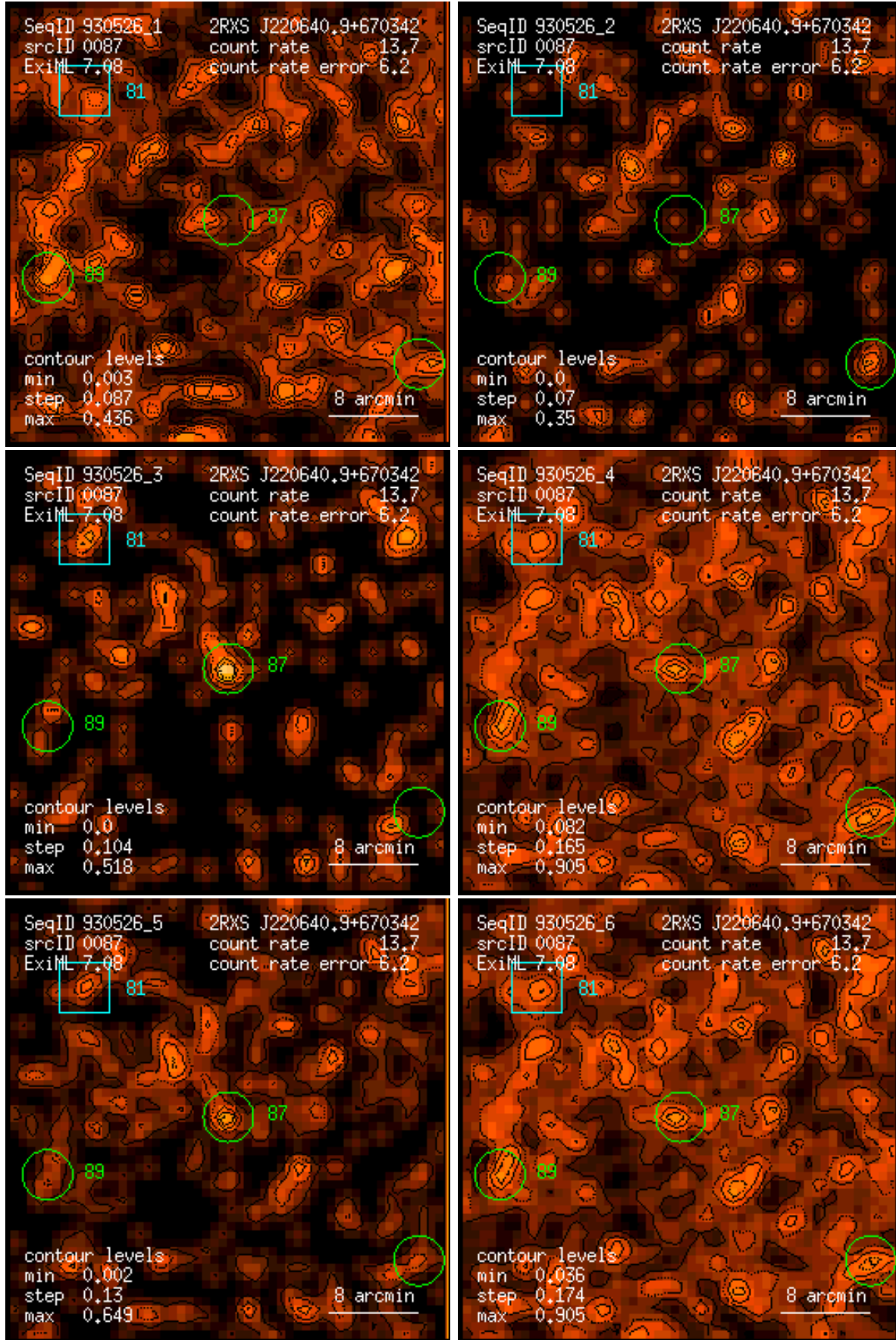
Figure 87: RASS 930526: detection 0087: band rate images, Gaussian filter: (1) PSPC channels 11 – 41, (2) 52 – 90, (3) 91 – 201, (4) 11 – 235, (5) 52 – 201, (6) 11 – 201. Broad band rates in counts/ks. Band rate contour levels in counts/ks/arcmin 2 .
