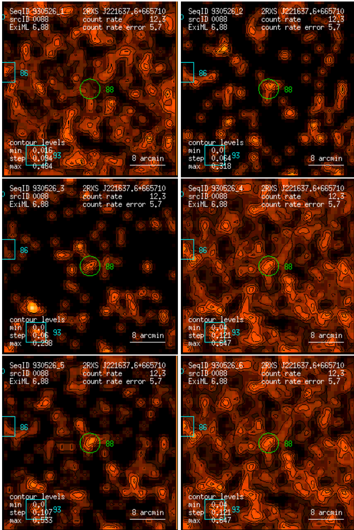
Figure 88: RASS 930526: detection 0088: band rate images, Gaussian filter: (1) PSPC channels 11 – 41, (2) 52 – 90, (3) 91 – 201, (4) 11 – 235, (5) 52 – 201, (6) 11 – 201. Broad band rates in counts/ks. Band rate contour levels in counts/ks/arcmin 2 .
