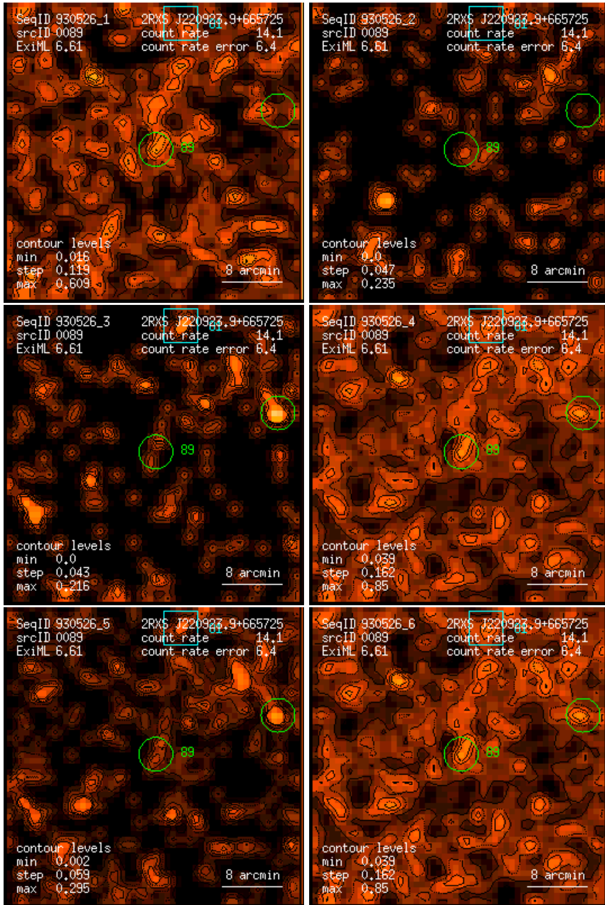
Figure 89: RASS 930526: detection 0089: band rate images, Gaussian filter: (1) PSPC channels 11 – 41, (2) 52 – 90, (3) 91 – 201, (4) 11 – 235, (5) 52 – 201, (6) 11 – 201. Broad band rates in counts/ks. Band rate contour levels in counts/ks/arcmin 2 .
