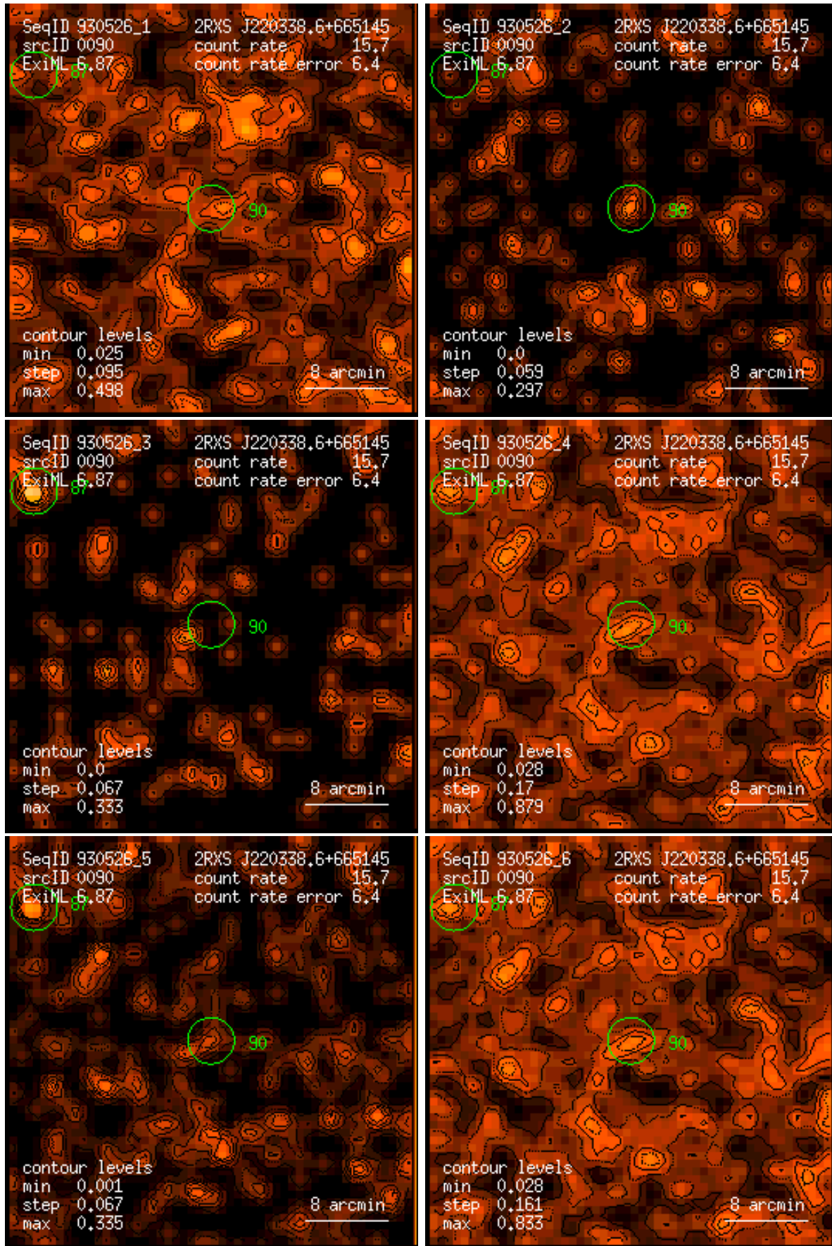
Figure 90: RASS 930526: detection 0090: band rate images, Gaussian filter: (1) PSPC channels 11 – 41, (2) 52 – 90, (3) 91 – 201, (4) 11 – 235, (5) 52 – 201, (6) 11 – 201. Broad band rates in counts/ks. Band rate contour levels in counts/ks/arcmin 2 .
